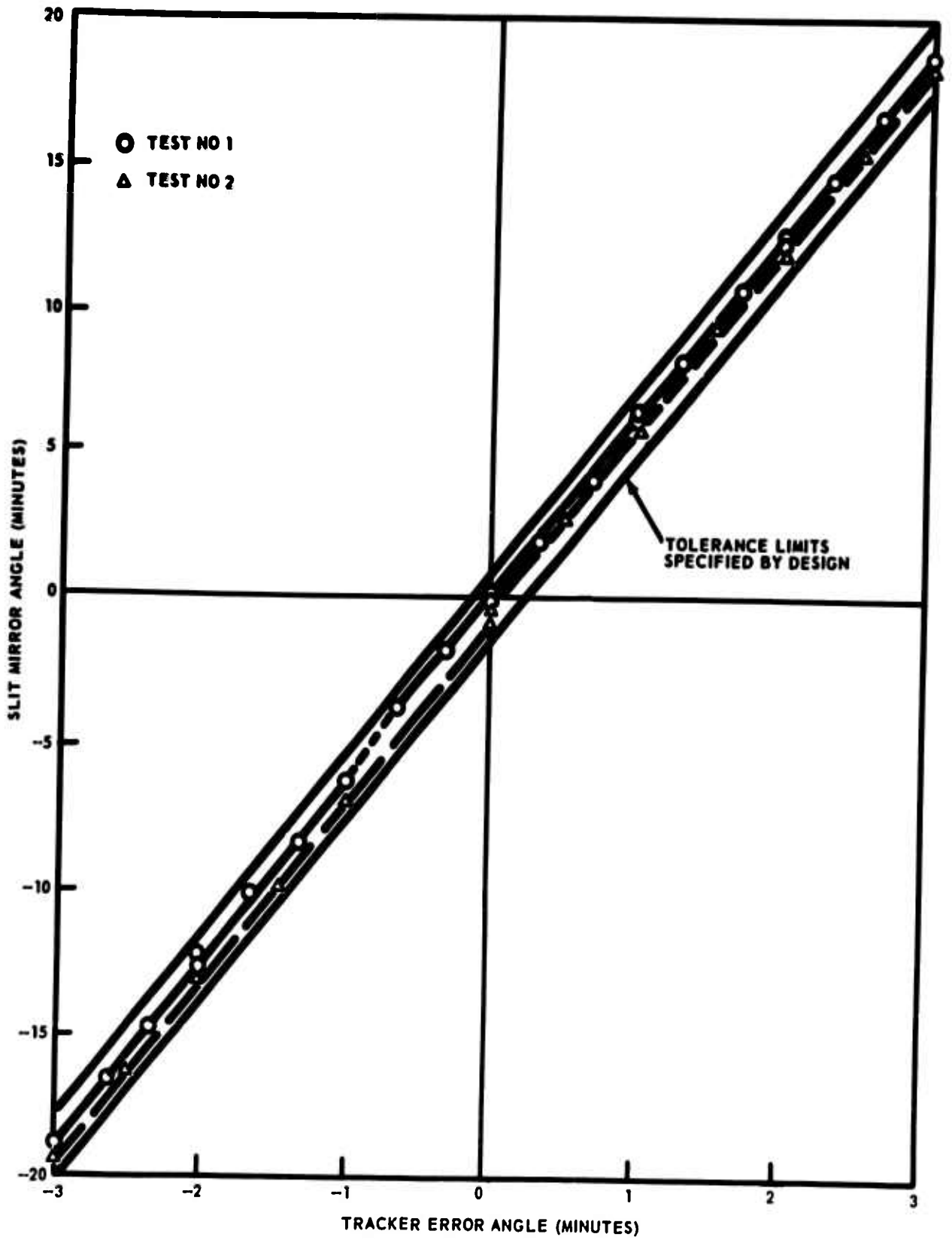
Figure 4-1B Slit Mirror Azimuth Angle vs Tracker Azimuth Error Angle
