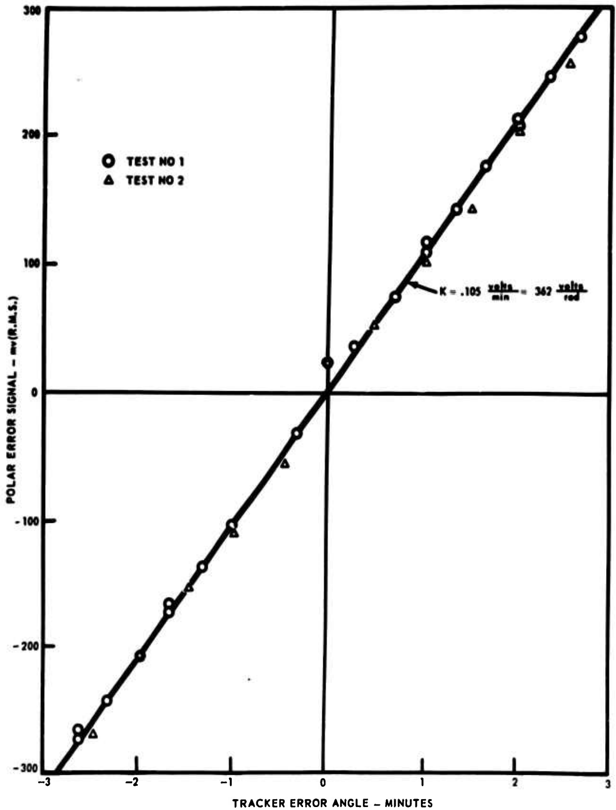
Figure 4-3A Polar Error Signal (Track) vs Tracker Elevation Error Angle
