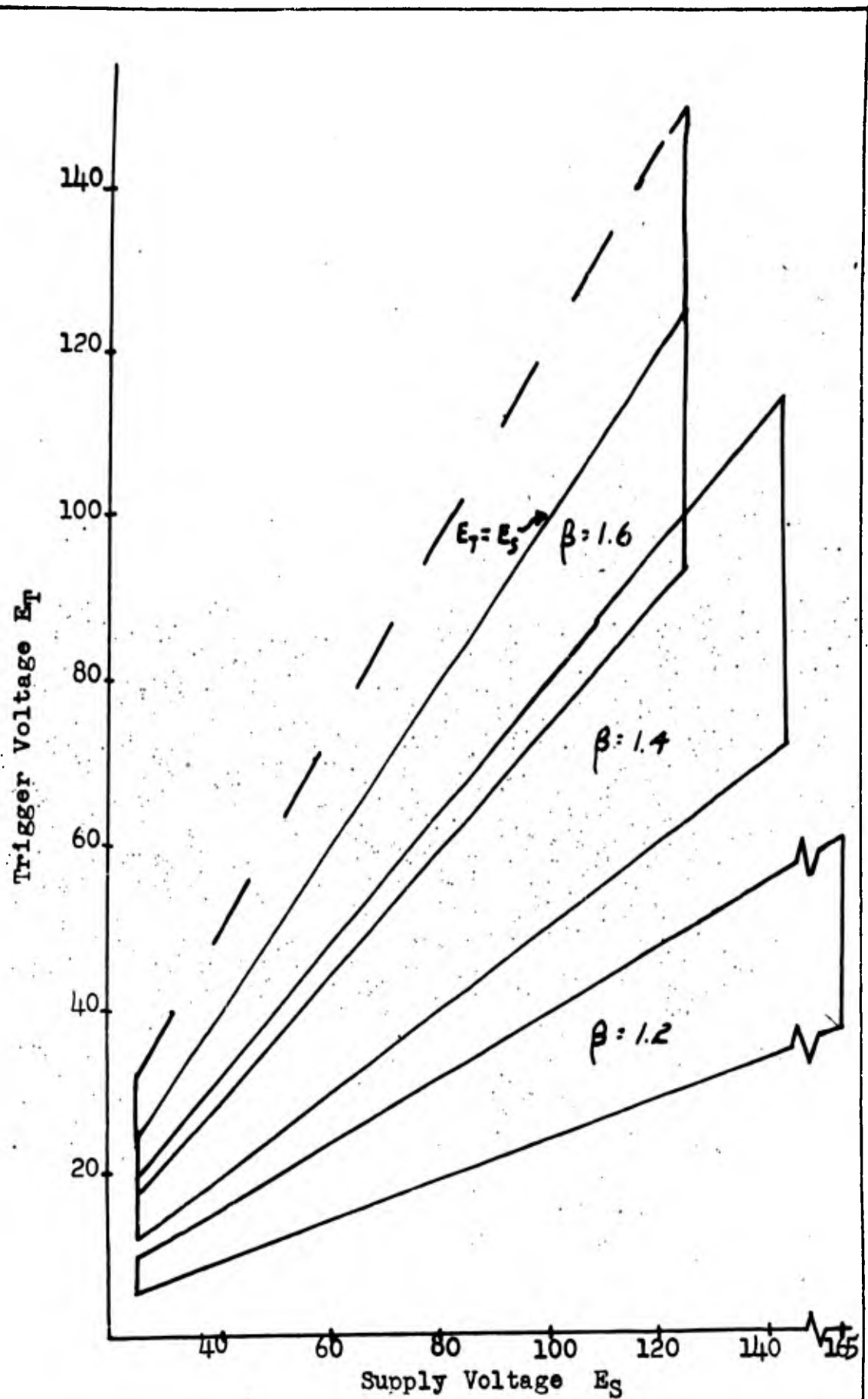
Fig. 9 Voltage Levels Possible For Various Values Of \beta
