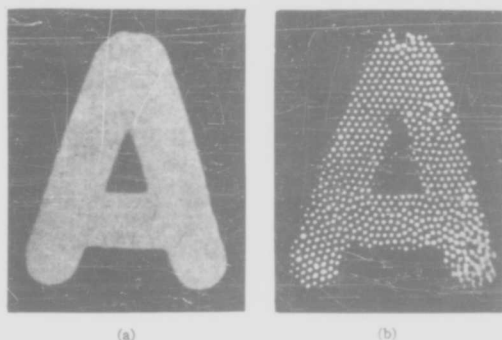
FIG. 11. Illustrating the imaging capability of a 1\text{-}\mu fiber bundle (N.A. = 1.15) (a) test object and (b) image of test object.
