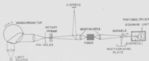
FIG. 6. Optical setup for investigating waveguide effects in isolated fibers and assemblies of fibers.
