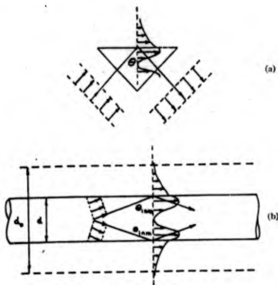
FIG. 1. Illustration of analogous interference and evanescent wave phenomena at (a) plane interface and (b) cylindrical fiber boundary.
