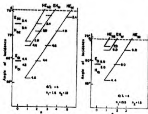
FIG. 3. Chart of solutions to the characteristic Eq. (7). Each bar represents a permissible mode. The m modes for a given n (abscissa) are arranged vertically, each at a height of its corresponding characteristic angle, given by the ordinate. The slanted lines connect modes of the same m number. The number inserted at the right of each bar gives the "optical diameter" of the fiber for that mode. (a) d/\lambda = 4 ; n_1 = 1.6 and (b) d/\lambda = 4 ; n_1 = 1.55 ; n_2 = 1.5 .
