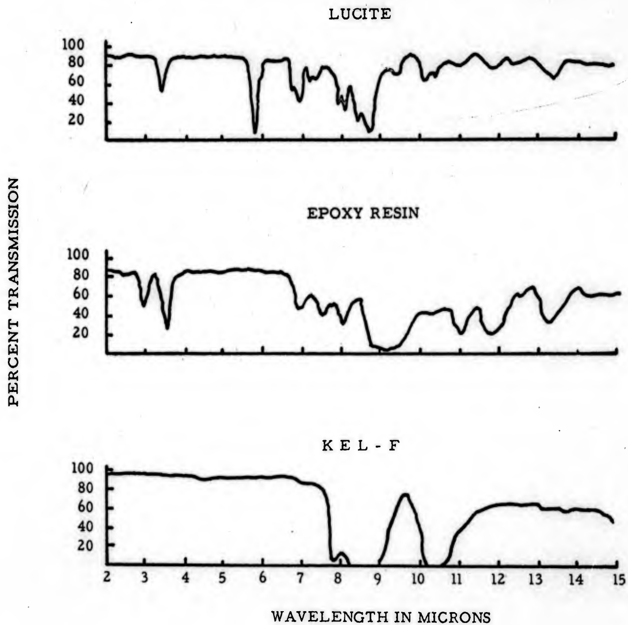
FIG. 4. INFRARED TRANSMISSION OF POTTING MATERIALS
