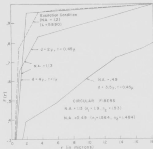
FIG. 8. "Flux passing through a hole" curves for point-spread functions of various fiber assemblies.
