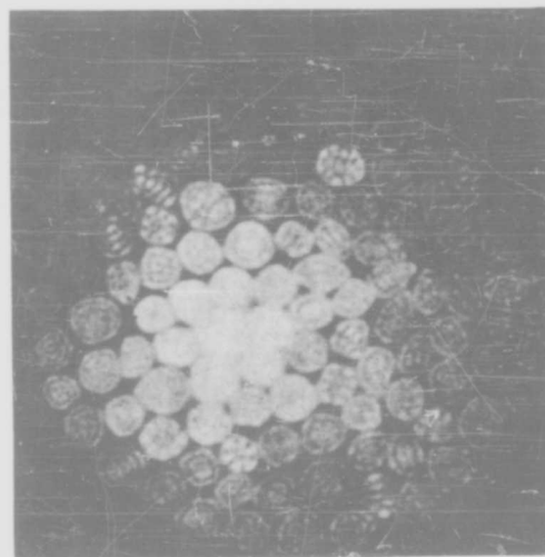
FIG. 7. Typical photomicrograph of exit end of a bundle, illustrating waveguide mode coupling when a single fiber is excited. ( d \approx 3\mu ; n_1 = 1.61 , n_2 = 1.52 .)
