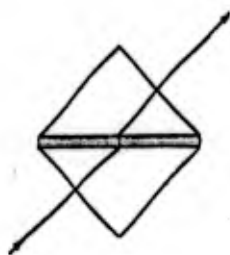
FIG. 5. Illustration of frustrated total reflection and energy coupling in a multilayer, frustrated-total-reflection filter.
