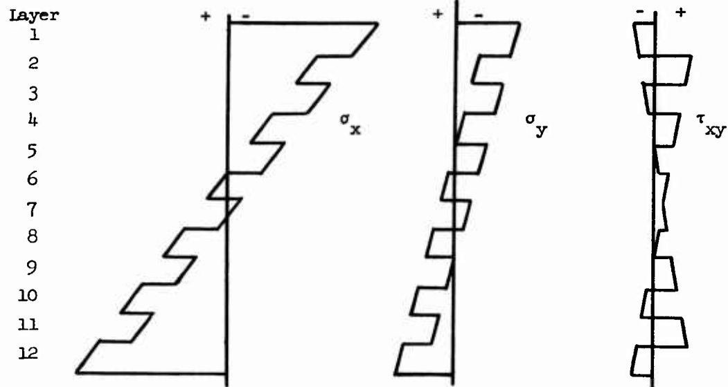
Figure 5.7 Typical Stress Distributions for Cylindrical Bending by a Uniform Moment and Uniformly Distributed Load
