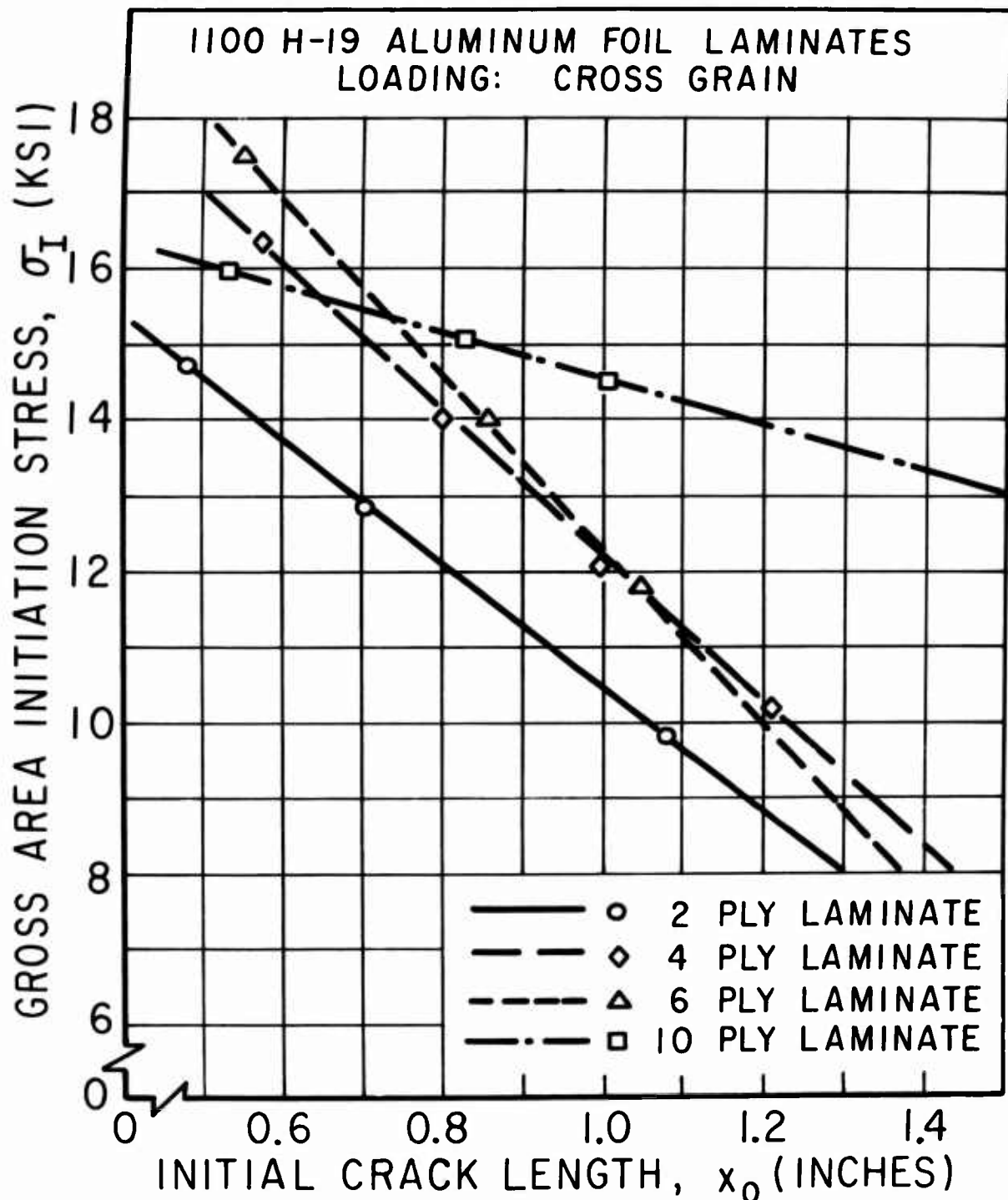
Figure 8b. Gross Area Initiation Stress vs Initial Crack Length in 1100 H-19 Aluminum Foil Laminates
