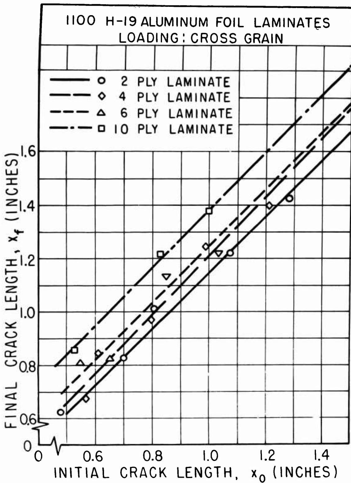
Figure 7b. Final Crack Length vs Initial Crack Length in 1100 H-19 Aluminum Foil Laminates
