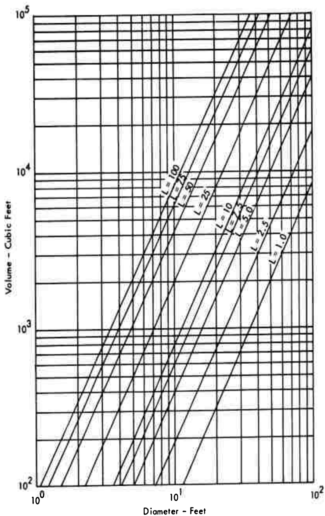
FIGURE III-26 CYLINDER VOLUME VS DIAMETER
