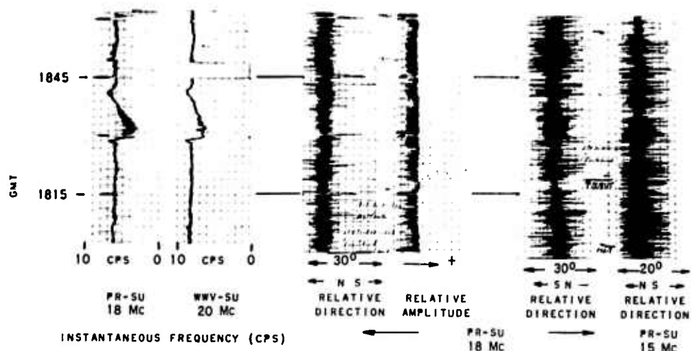
FIG. 19. FREQUENCY ANALYSIS OF TOTAL RECEIVED FREQUENCY SPECTRUM OF FREQUENCY FLUCTUATION CAUSED BY SI, 4 FEBRUARY 1961. FREQUENCIES OF THE MANY INCOMING MODES AFFECTED BY DIFFERENT AMOUNTS SIMULTANEOUSLY OVER WIDELY SEPARATED PATHS.
