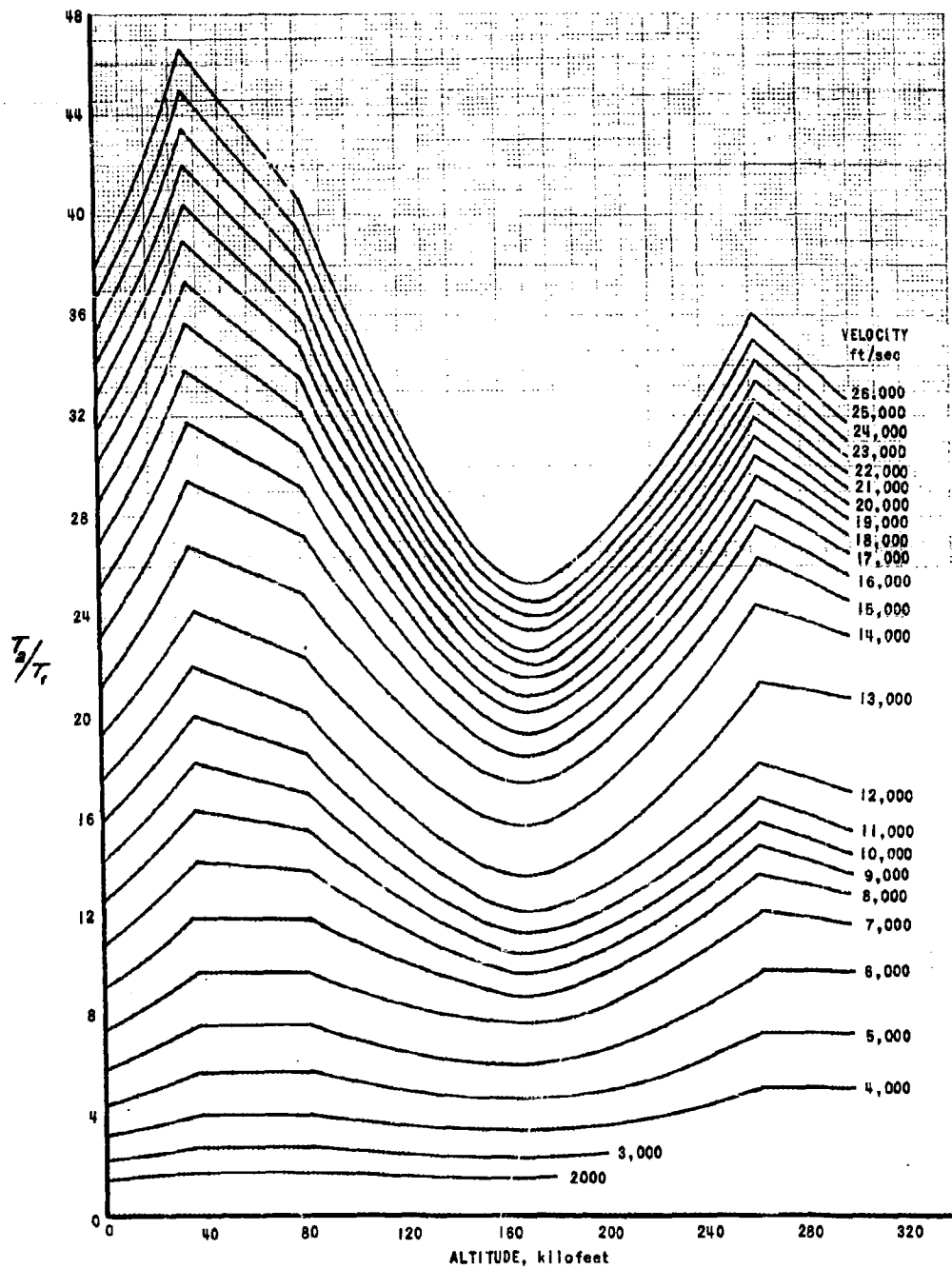
Graph 3 TEMPERATURE RATIO AS A FUNCTION OF ALTITUDE
