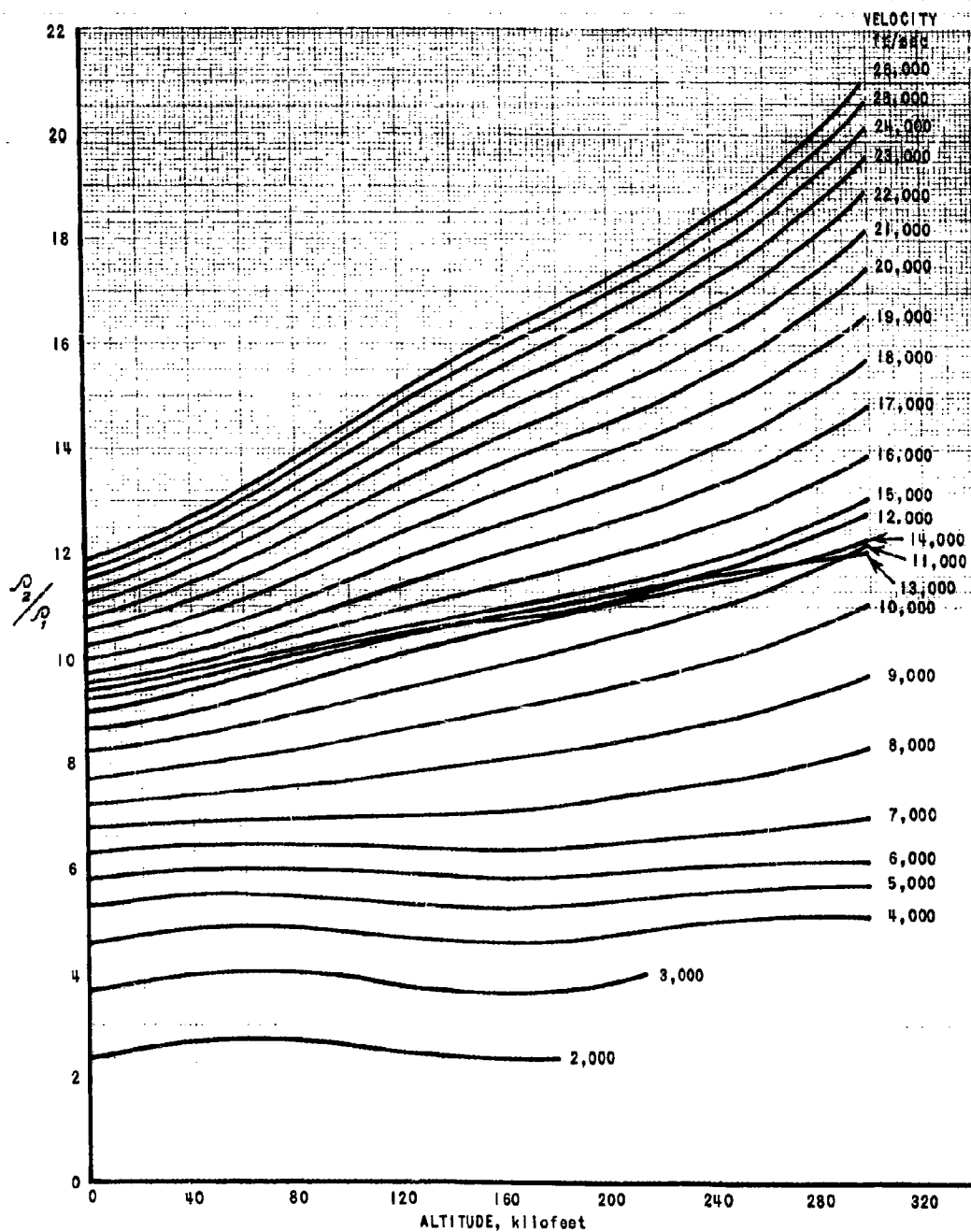
Graph 1 DENSITY RATIO AS A FUNCTION OF ALTITUDE
