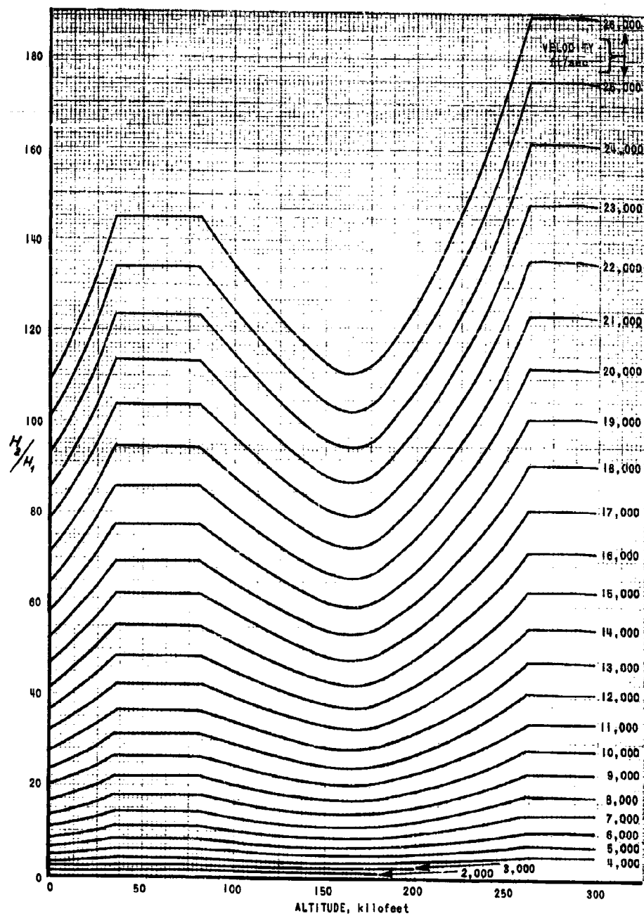
Graph 4 ENTHALPY RATIO AS A FUNCTION OF ALTITUDE
