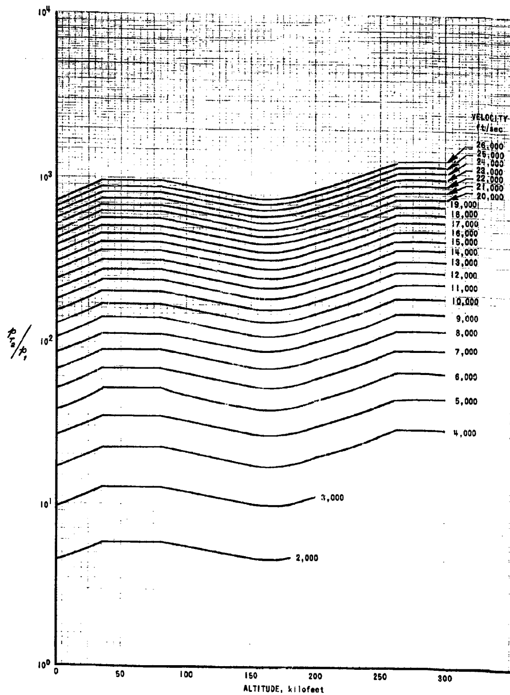
Graph 5 STAGNATION-POINT PRESSURE RATIO AS A FUNCTION OF ALTITUDE
