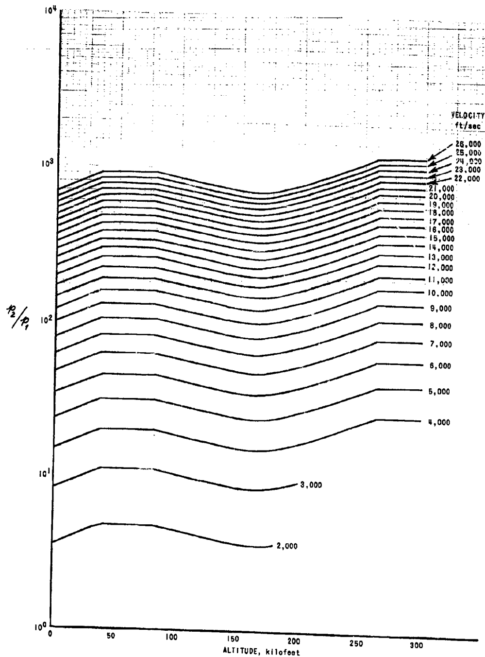
Graph 2 PRESSURE RATIO AS A FUNCTION OF ALTITUDE
