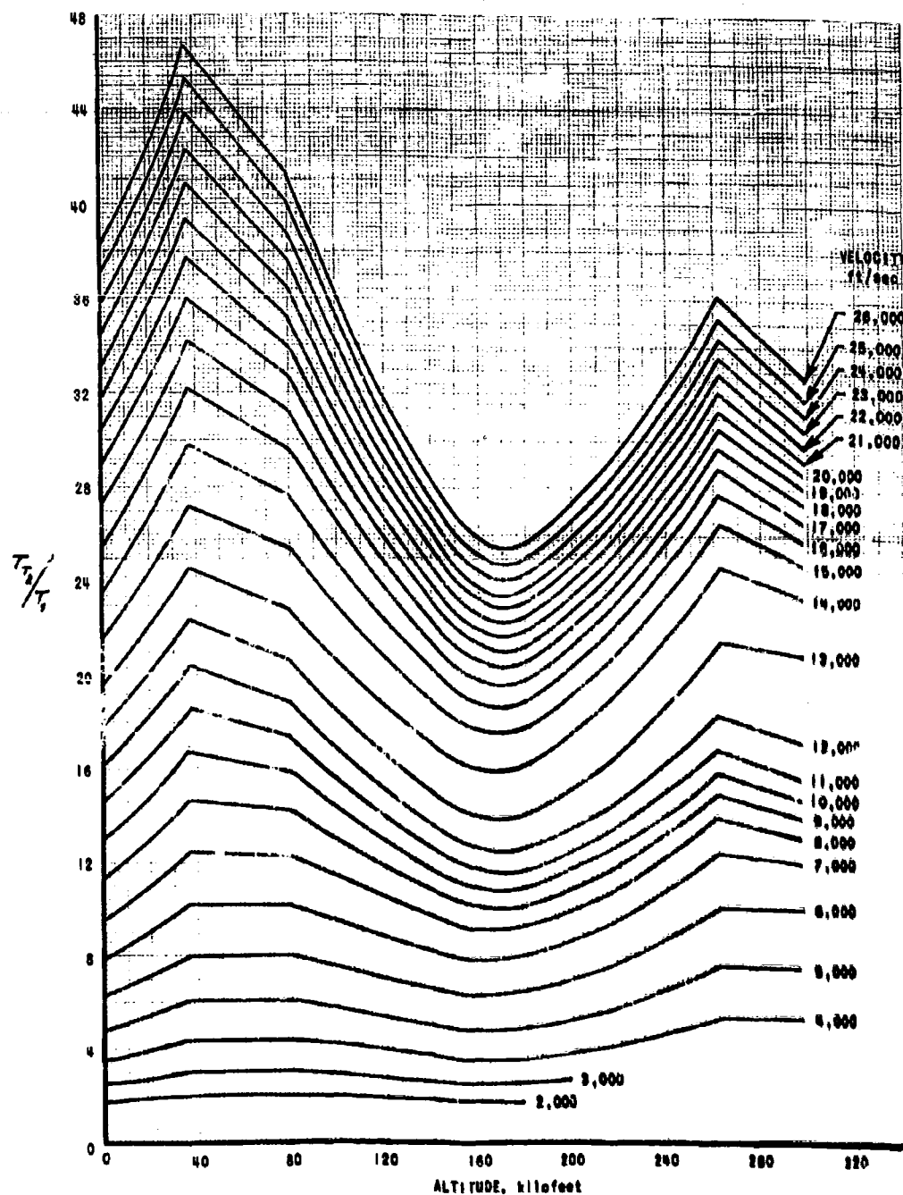
Graph 6 STAGNATION-POINT TEMPERATURE AS A FUNCTION OF ALTITUDE
