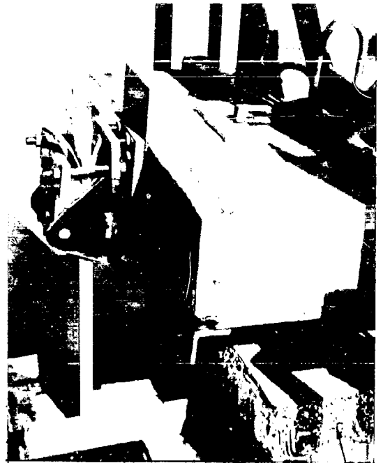
PAPER HONEYCOMB PADS PLACED AS A SAFETY DEVICE IN PRELIMINARY DROPS IN EVENT OF FAILURE OF WOOD.
