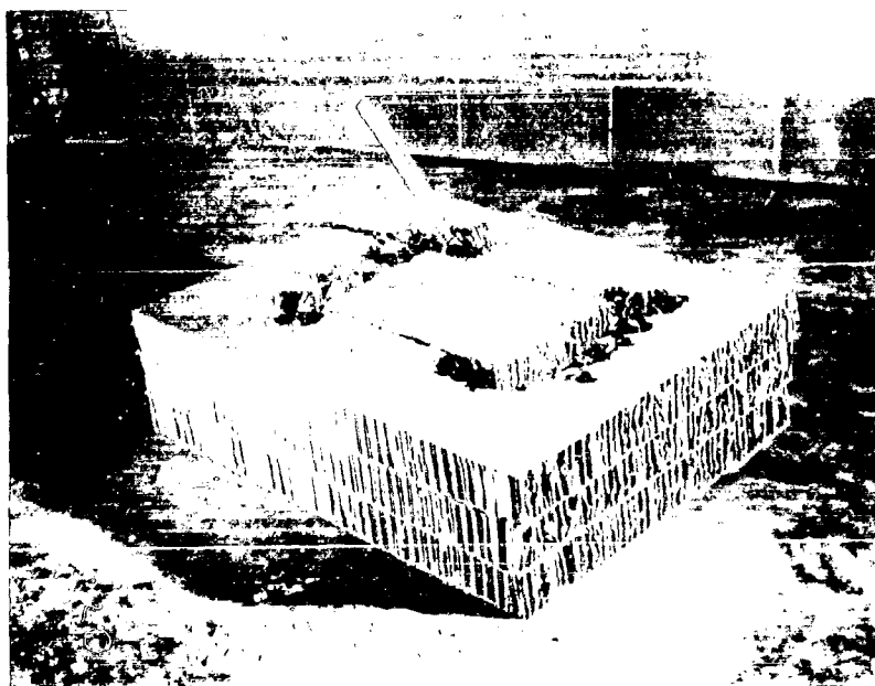
Fig. 7.15. Precrushing Honeycomb Around the Wheel Crushing Area
