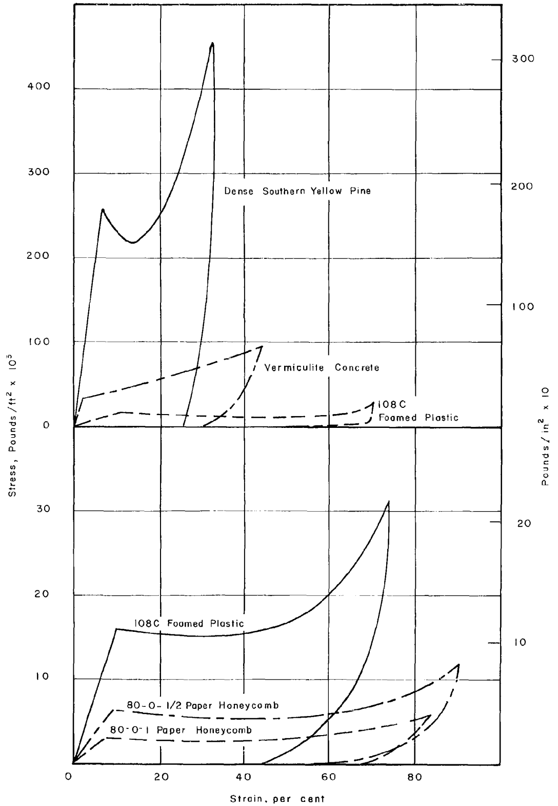
Fig. 2.2. Typical Dynamic Stress-Strain Curves of Materials Under Compression Loads
