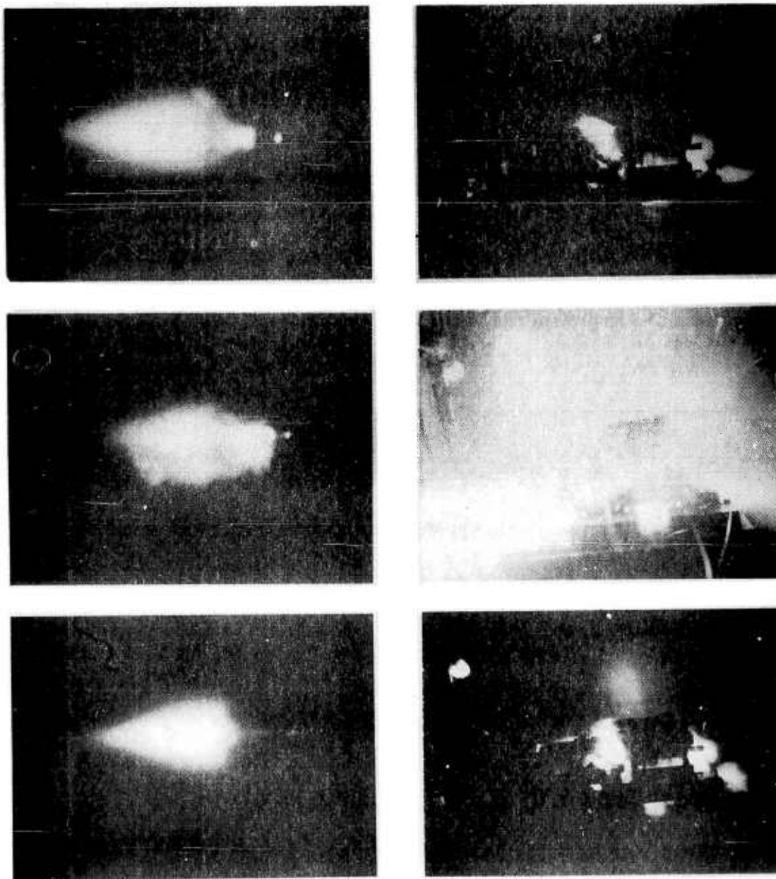
Test of M52A3B1 Primer and WC 870 Propellant. Cumulative flash produced by a 125 round burst fired from a 20 mm M39A2 gun. Top fired at +70° F; Center fired at +165° F; Bottom fired at -65° F.
