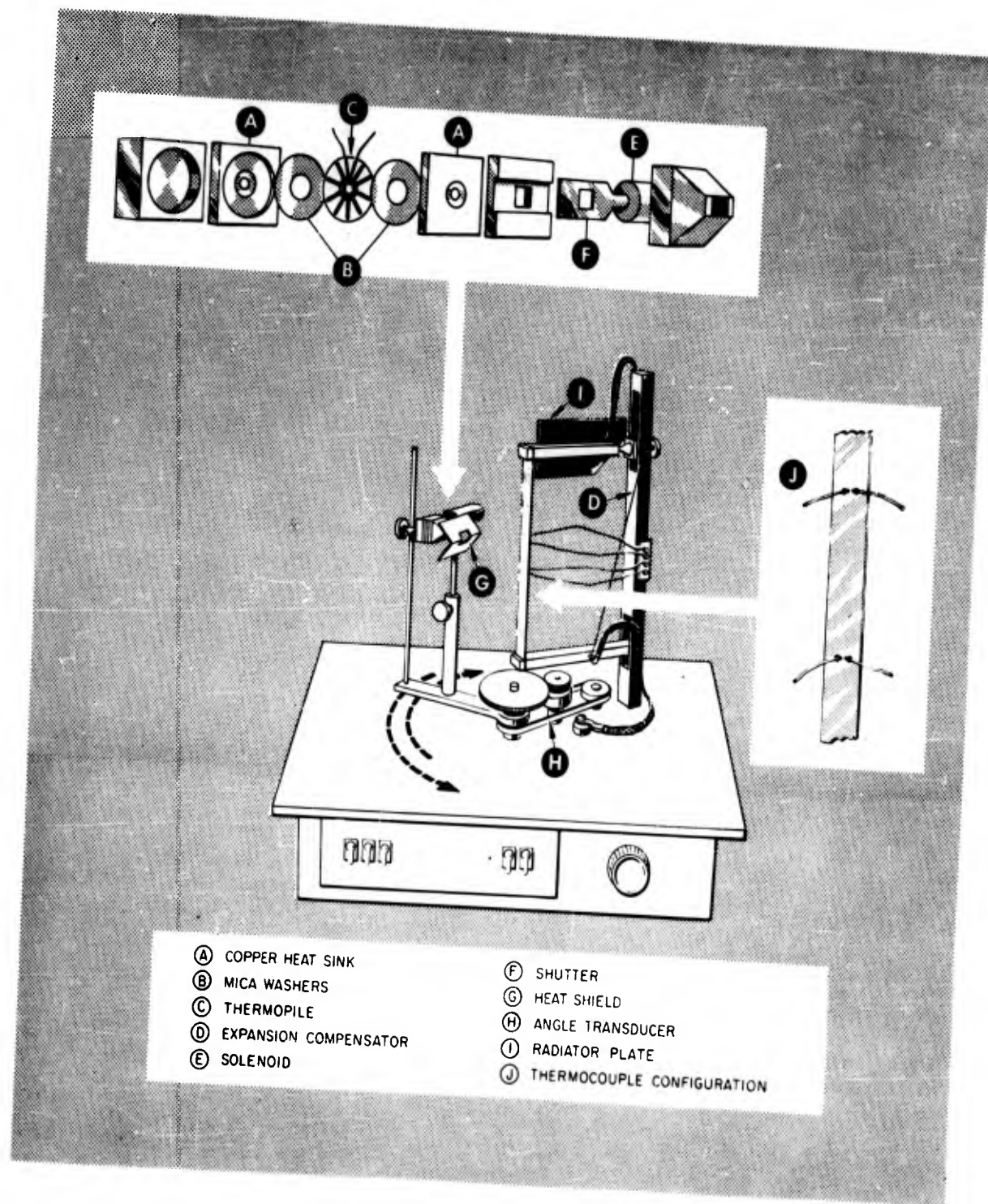
Fig. 1 Schematic diagram of experimental arrangement for measuring angular distribution.
