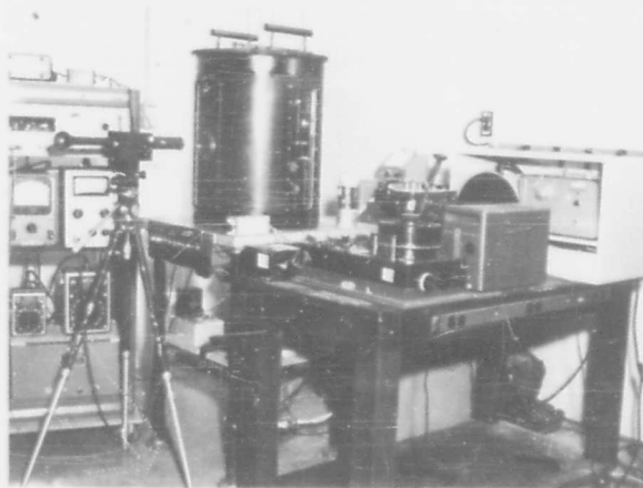
Fig. 3 Over-all photograph of apparatus for measurement of angular distribution.
