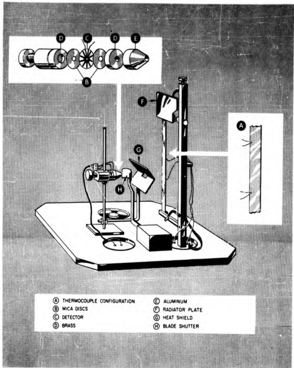
Fig. 4 Schematic diagram of experimental arrangement for measurement of time dependence of emittance.
