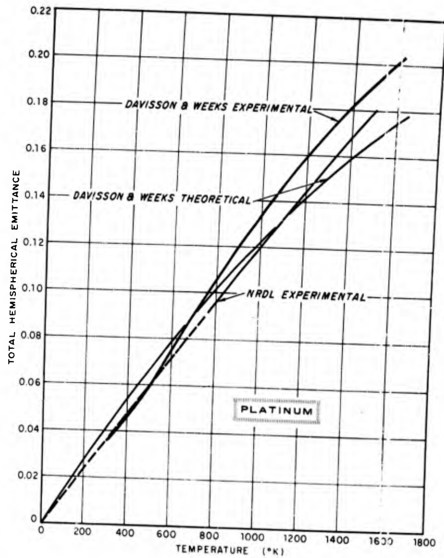
Fig. 23 Comparison of the total hemispherical emittance versus temperature measurements of Davisson and Weeks and NRDL.
