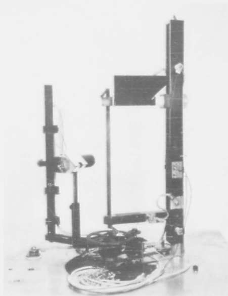
Fig. 2 Detail photograph of apparatus for measurement of angular distribution.
