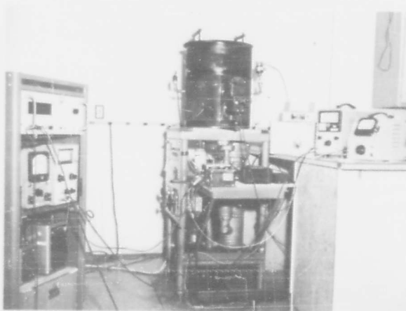
Fig. 6 Over-all photograph of apparatus for measurement of time dependence of emittance.
