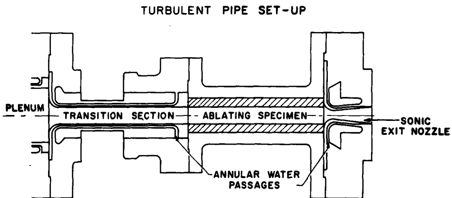
Fig. 3 Schematic Drawing of Experimental Equipment.
