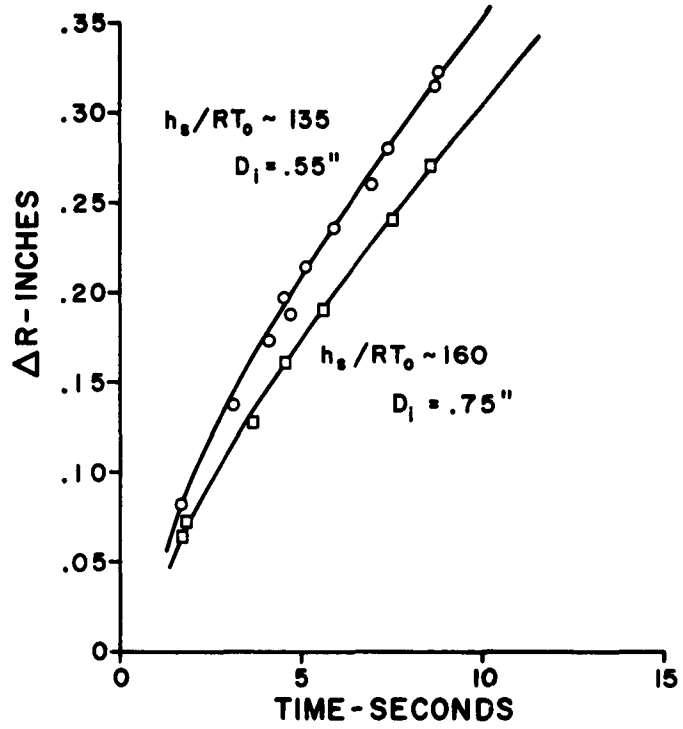
Fig. 5 Diameter Change of Teflon.
