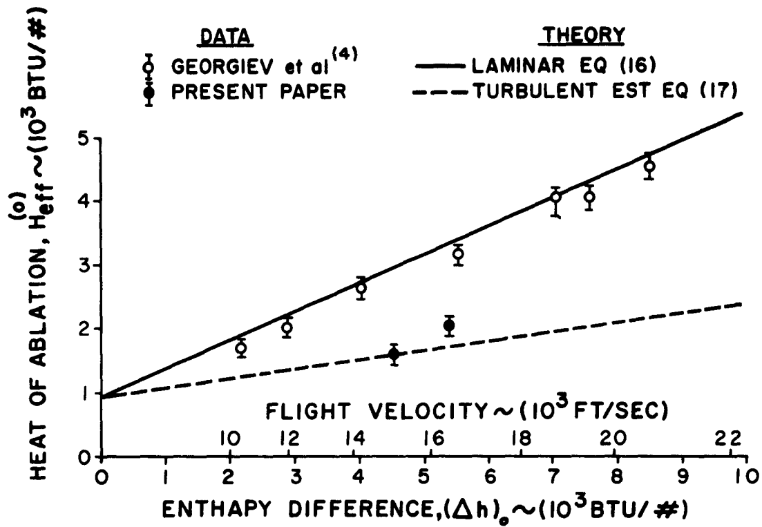
Fig. 7 Teflon Ablation.
