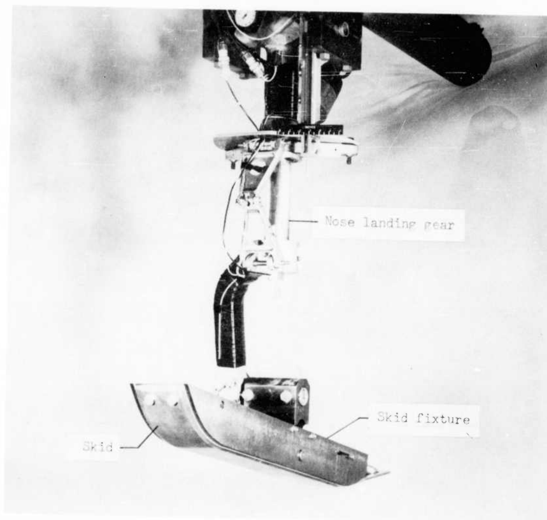
Figure 2.- Shoe skid attached to skid fixture for testing. L-59-1698.1
