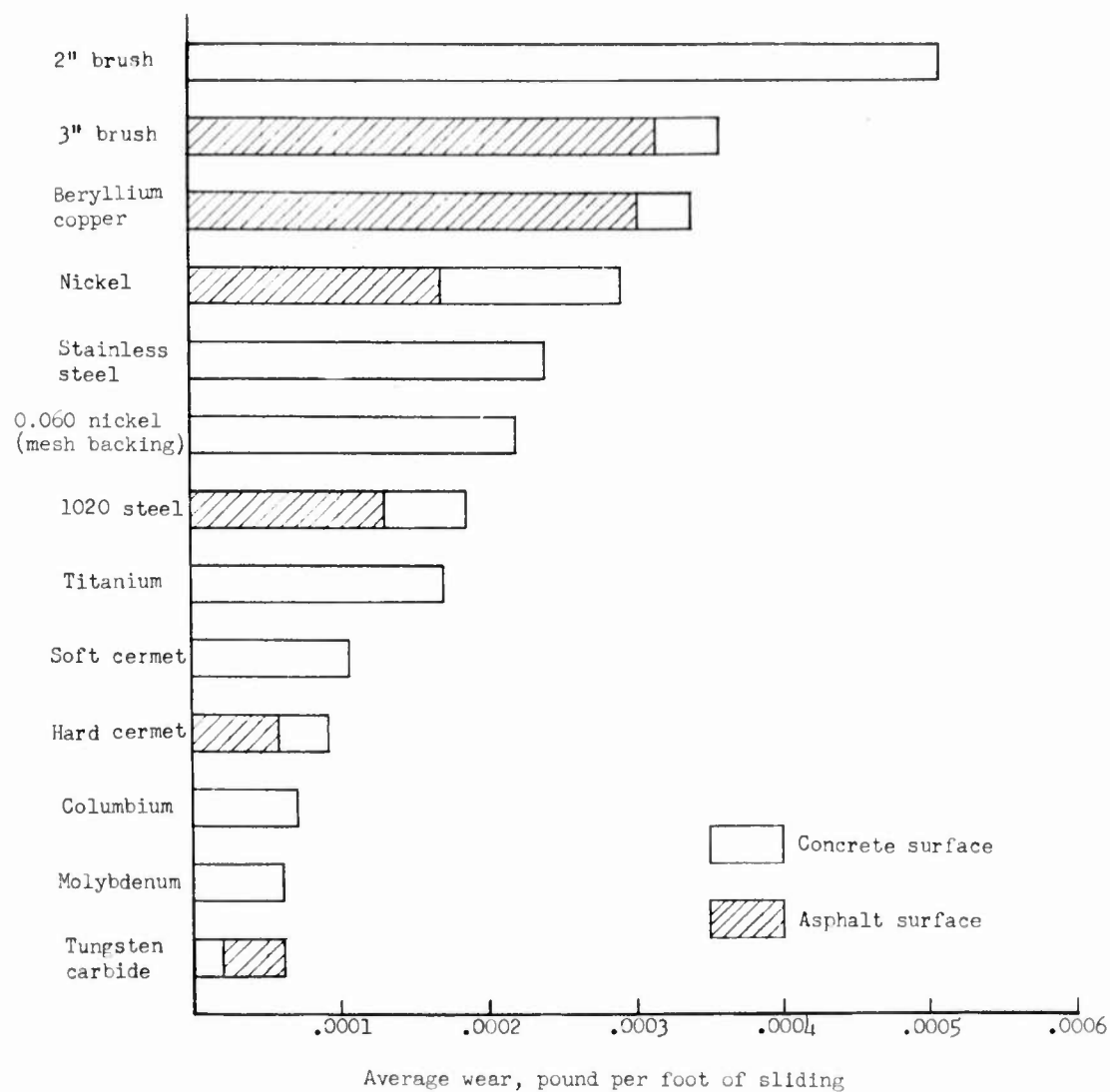
Figure 19.- Average wear of skids on concrete and asphalt surfaces. Static vertical load, 2,150 pounds.
