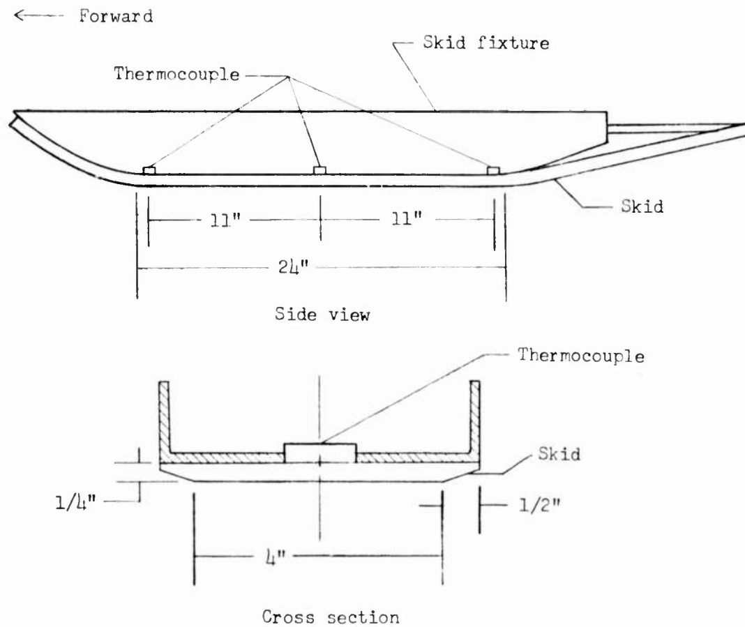
Figure 7.- Sketch showing locations of thermocouples on skid.
