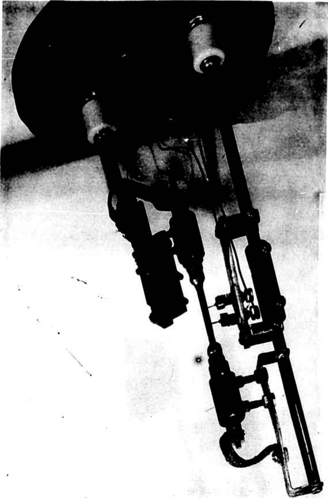
Figure 3. Sample Holder for Specific Heat Measurements
