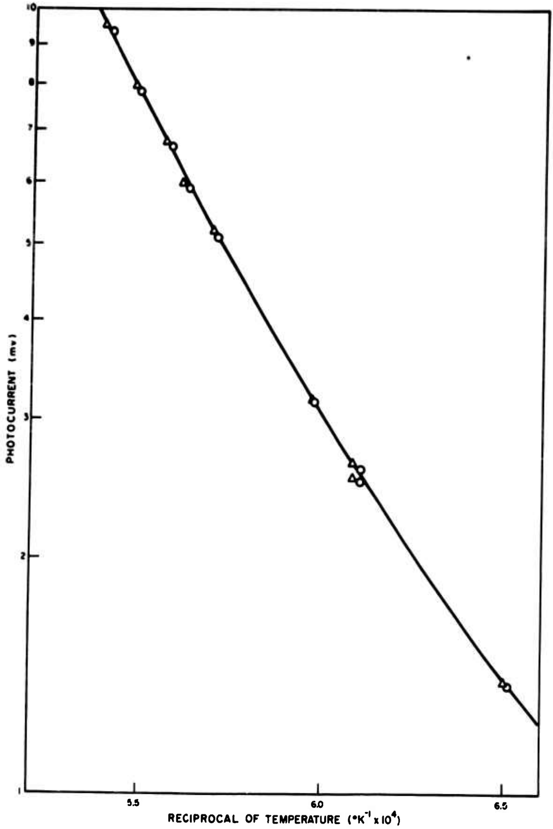
Figure 2. Calibration Curve of Photoelectric Pyrometer
