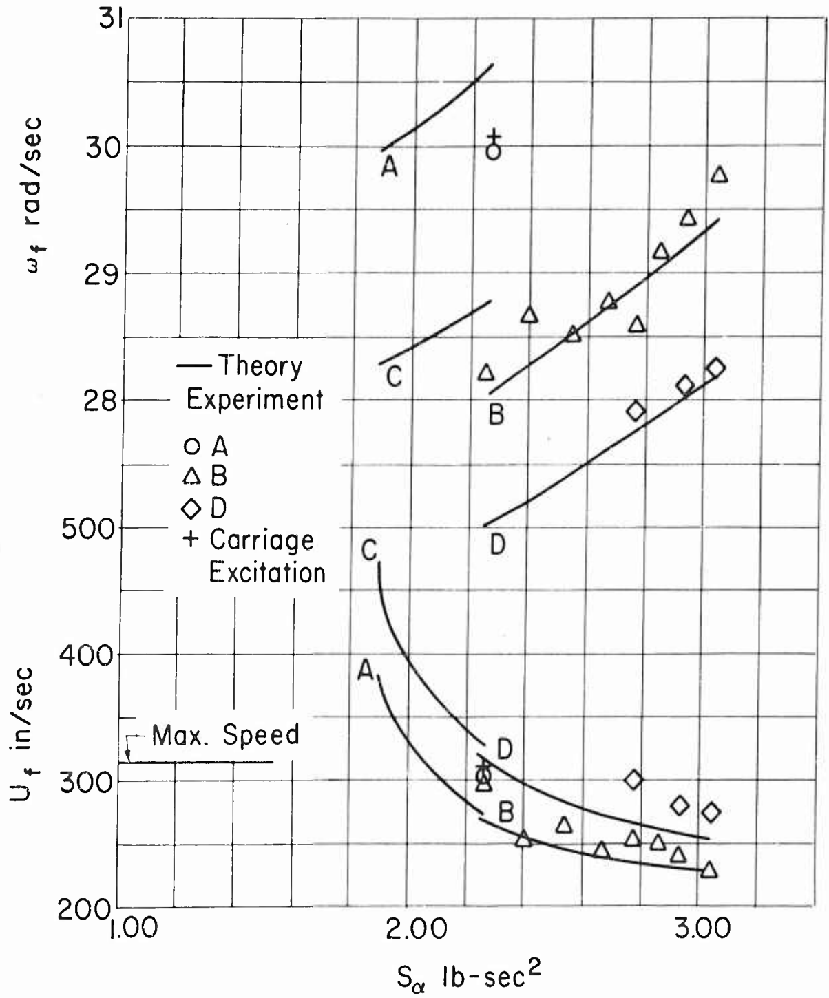
Figure 9 - Critical Speeds and Frequencies
