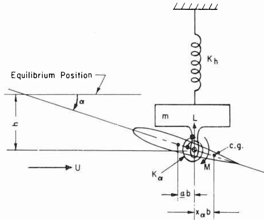
Figure 4 – Idealized Foil-Mass System
