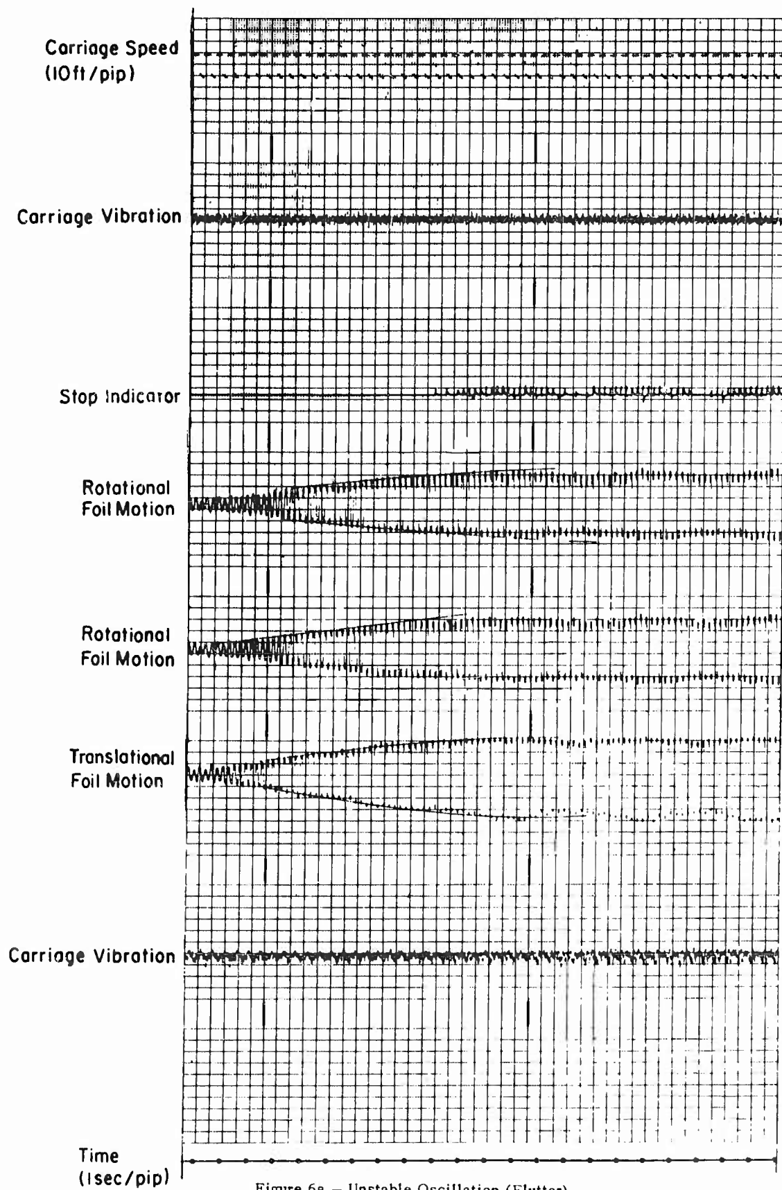
Figure 6a - Unstable Oscillation (Flutter) Complete Record
