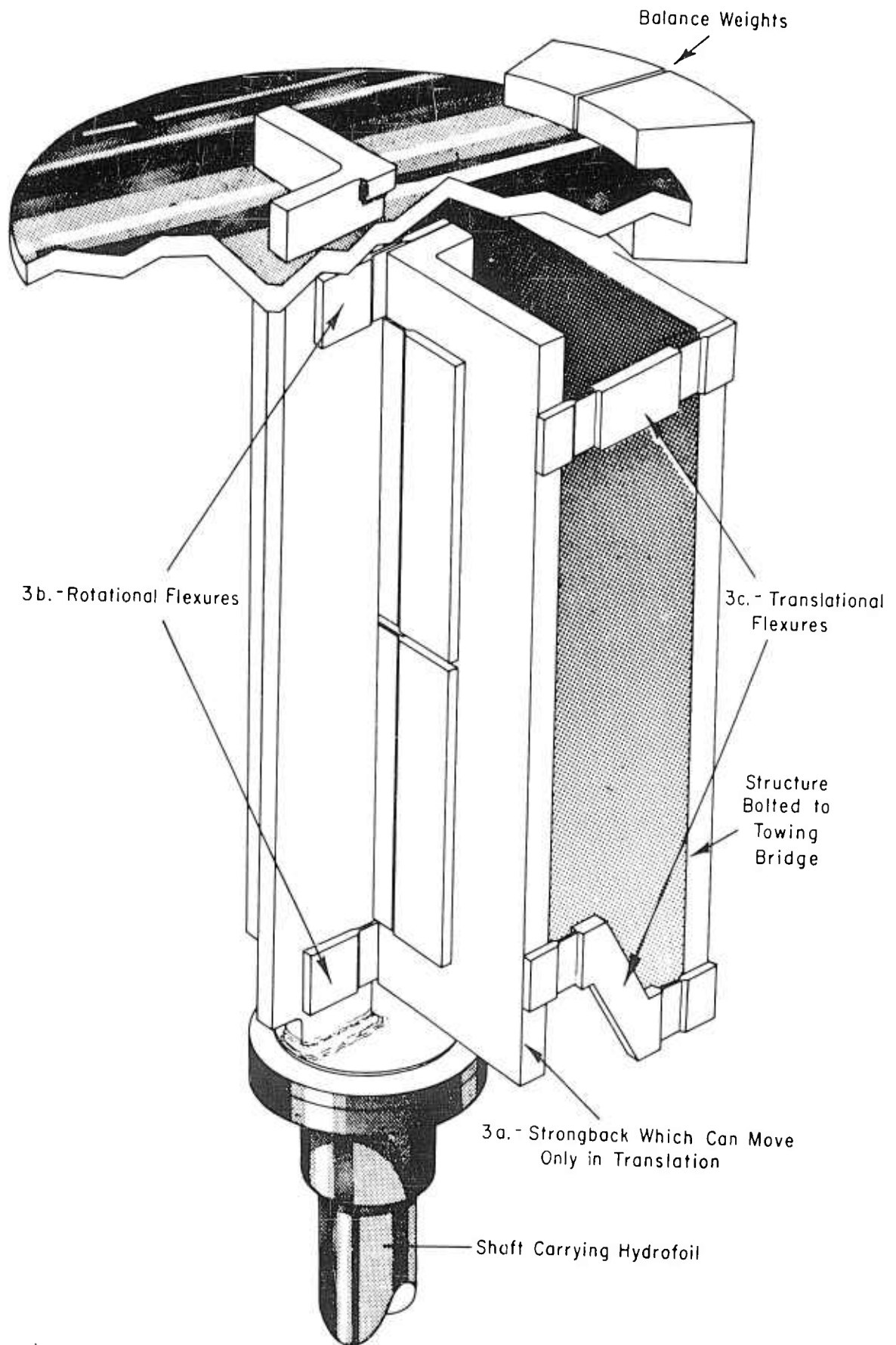
Figure 3 - Sectional Elevation of TMB Flutter Apparatus
