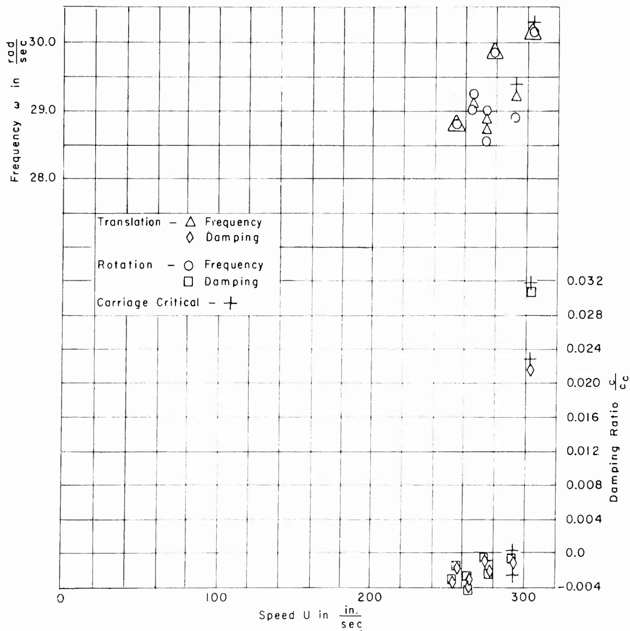
Figure 7h - Configuration B, S_{\alpha} = 2.66 \text{ lb-sec}^2
