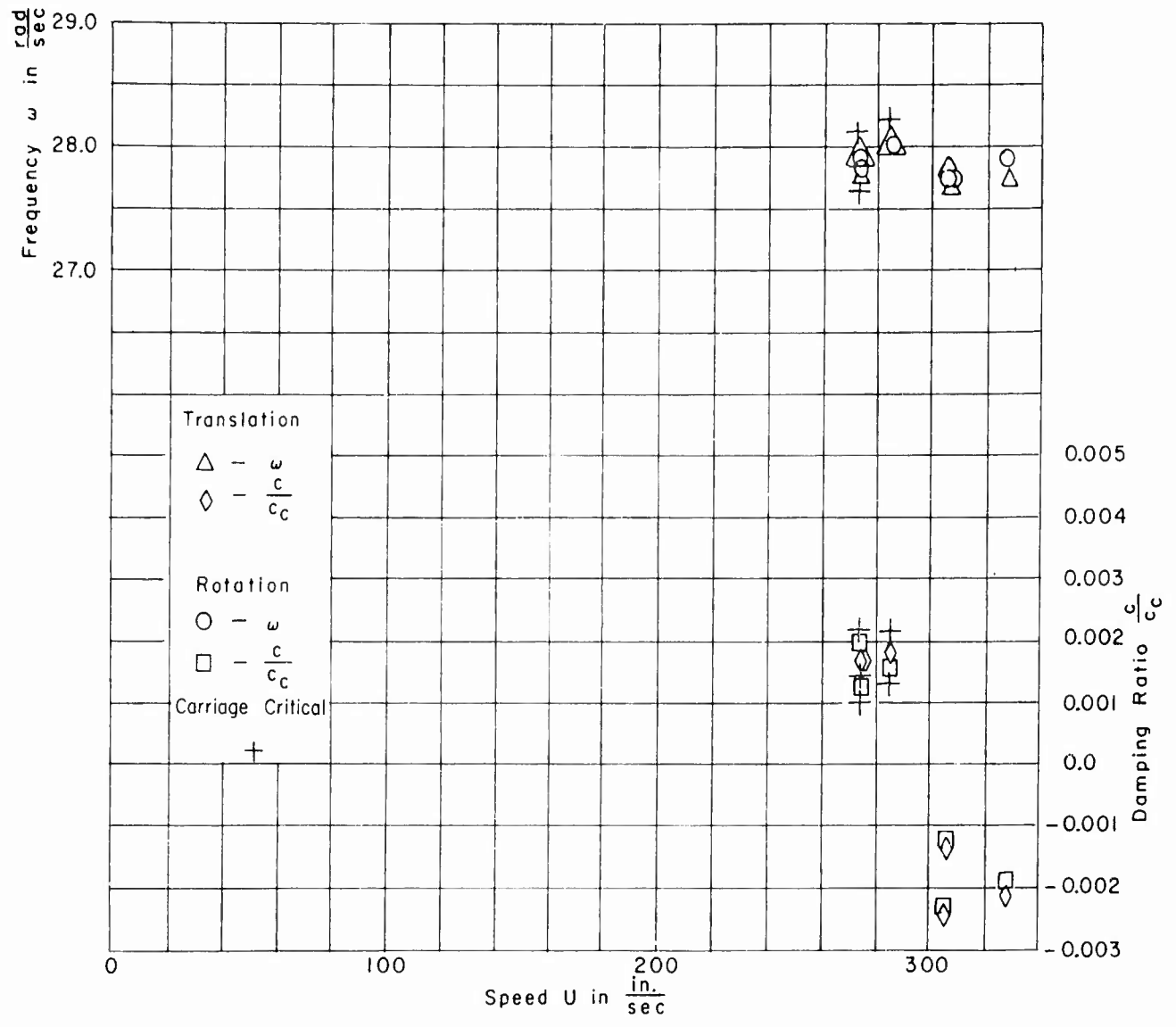
Figure 7u - Configuration D, S_{\alpha} = 2.77 \text{ lb-sec}^2
