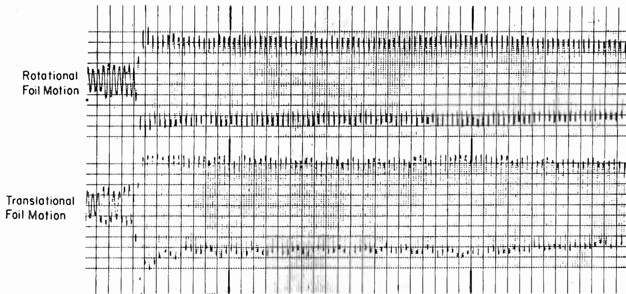
Figure 6c - Neutrally Stable Oscillation
