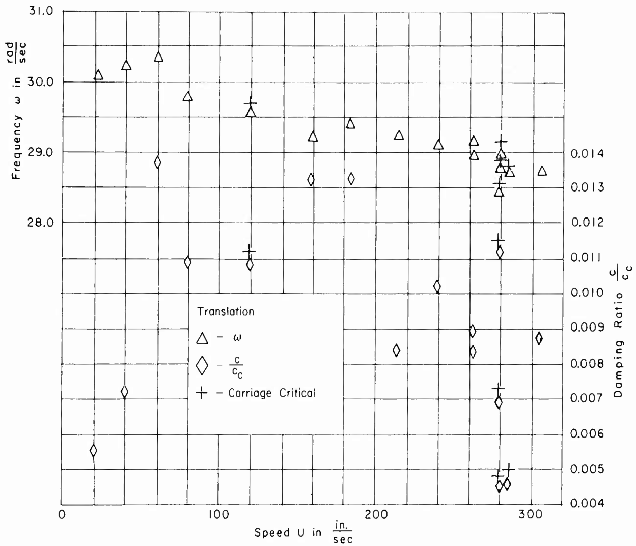
Figure 7t - Configuration C, S_{\alpha} = 2.26 \text{ lb-sec}^2 , Translation
