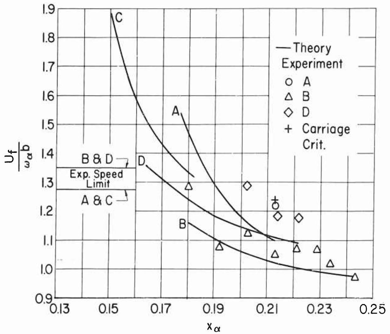
Figure 10 - Dimensionless Critical Flutter Parameters
