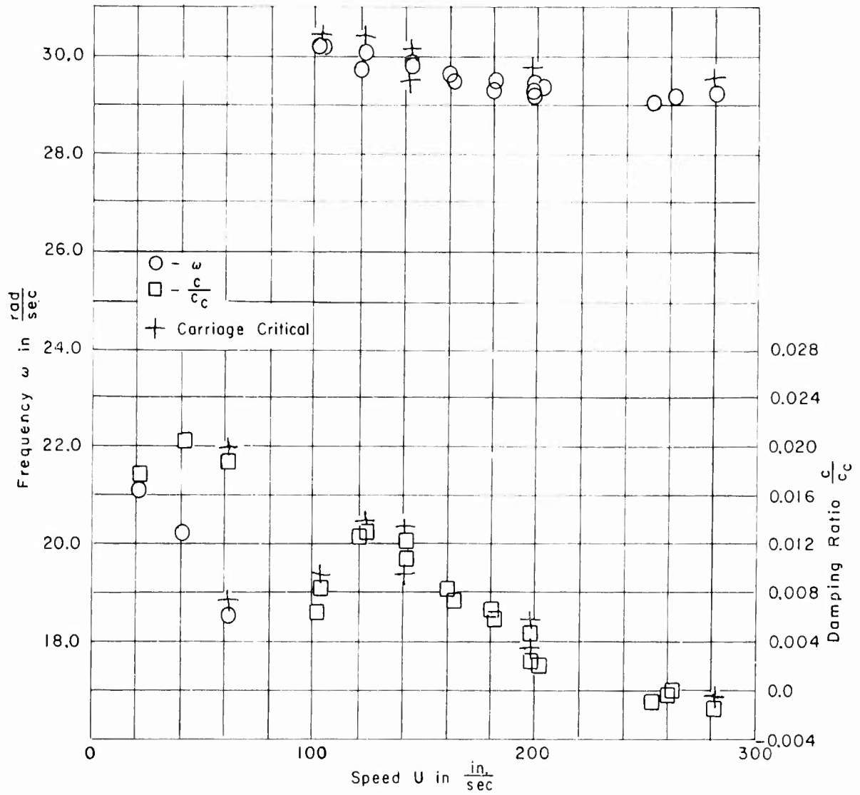
Figure 7i - Configuration B, S_{\alpha} = 2.77 \text{ lb-sec}^2 , Rotation
