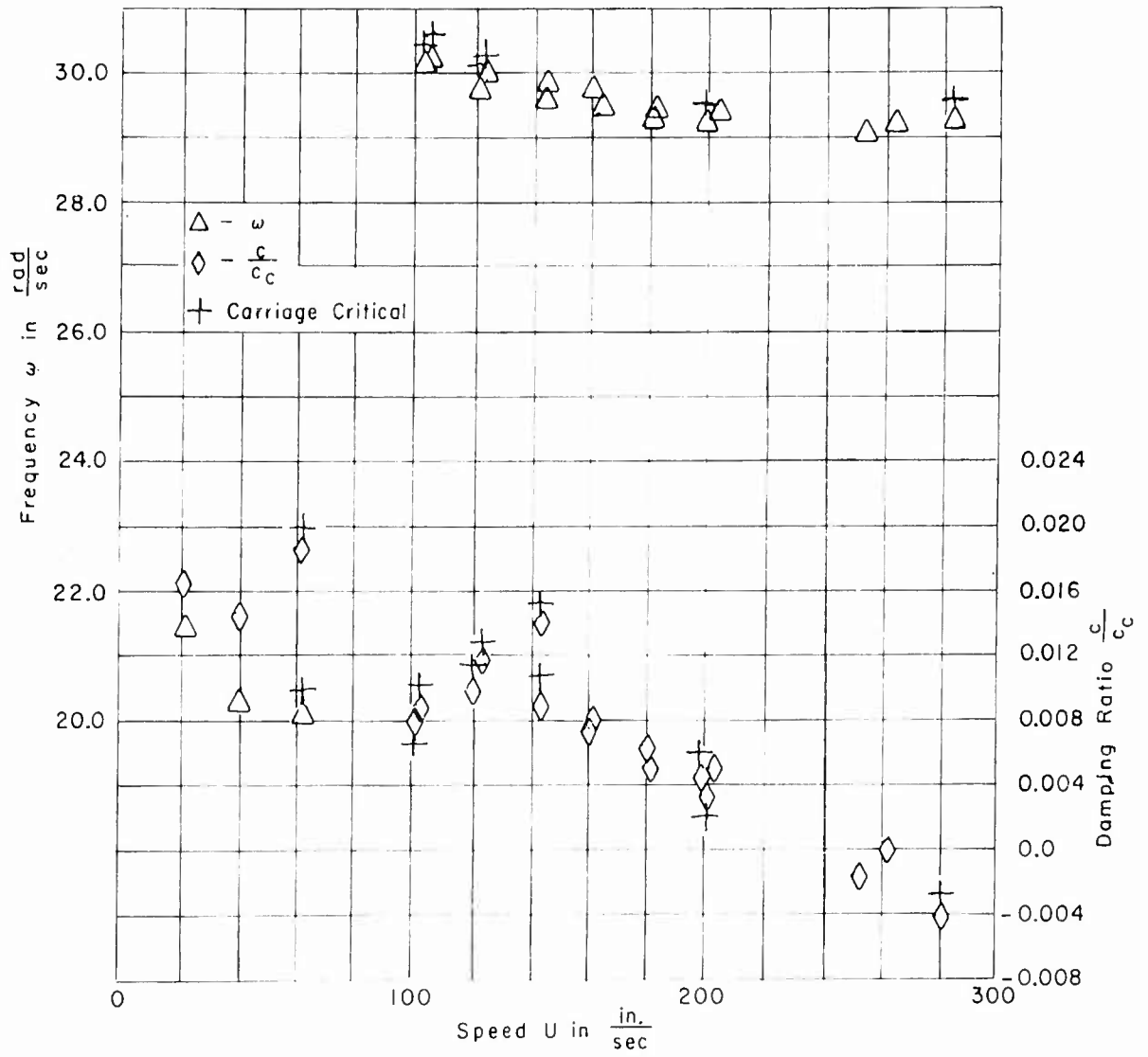
Figure 7j -- Configuration B, S_{\alpha} = 2.77 \text{ lb-sec}^2 , Translation
