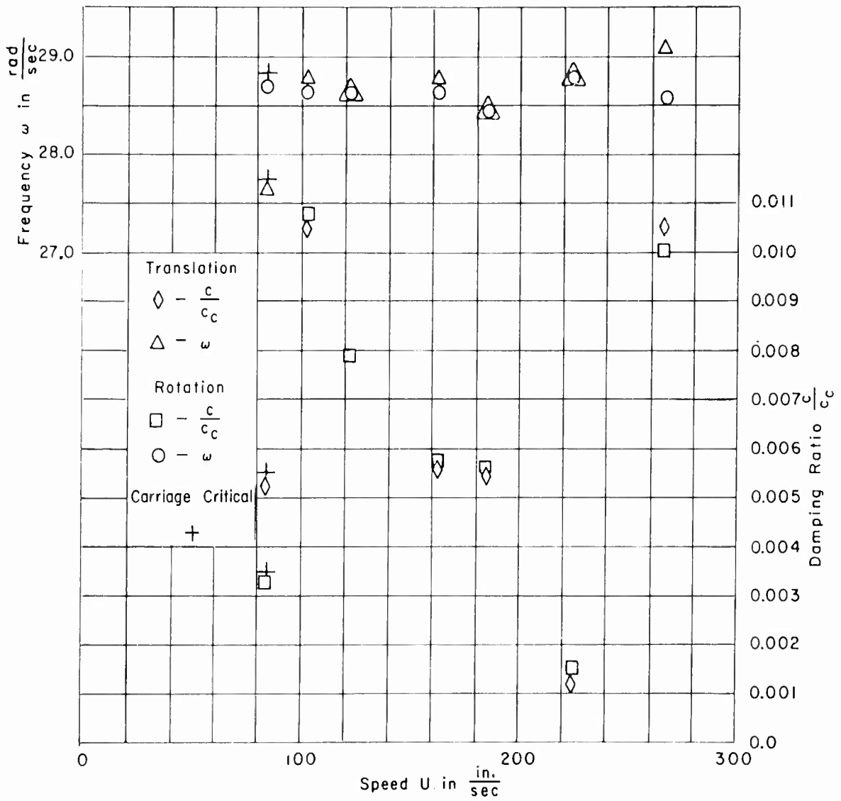
Figure 7c - Configuration B, S_{\alpha} = 2.25 \text{ lb-sec}^2 , \alpha_s = 0.6^\circ
