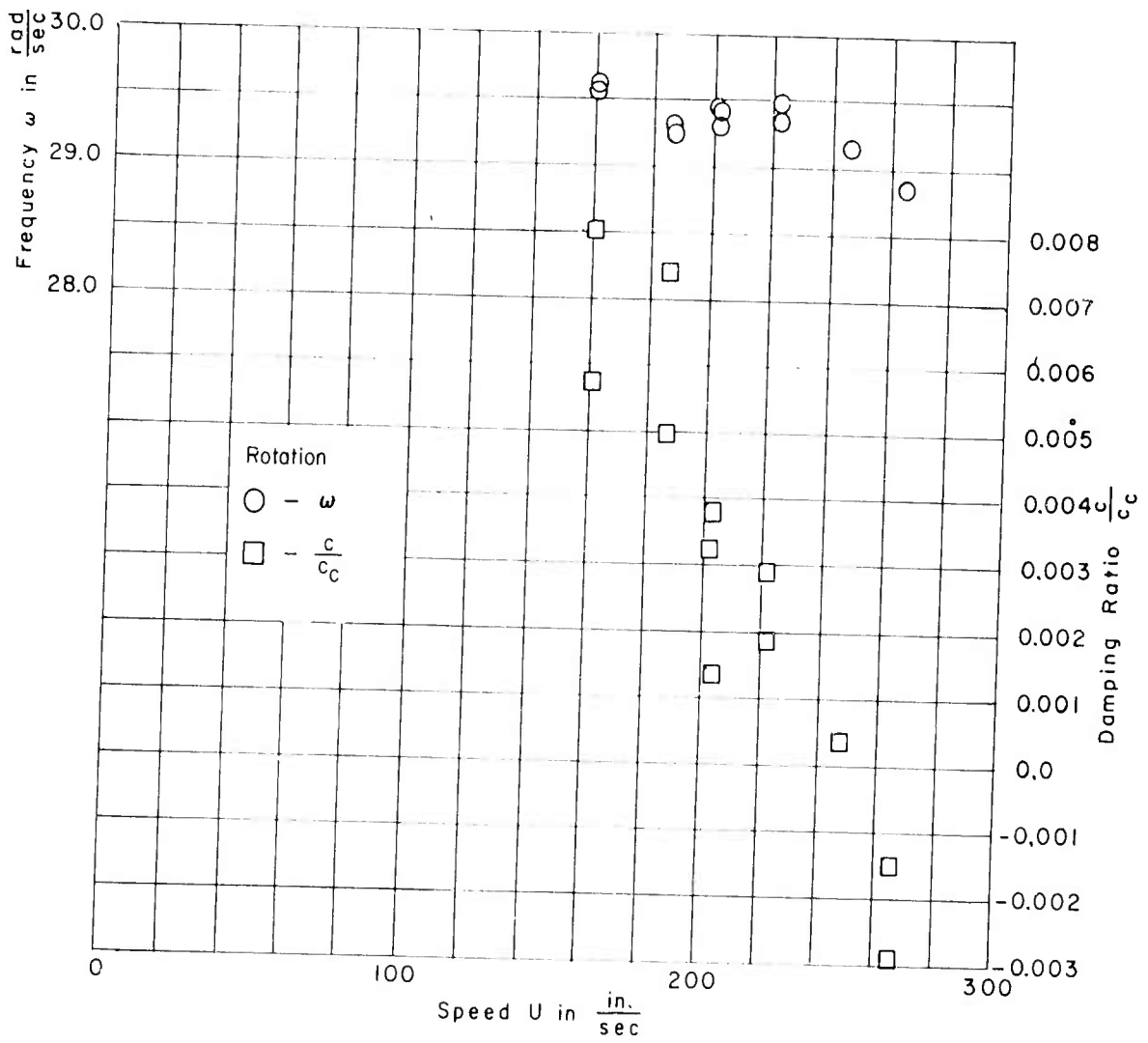
Figure 7k - Configuration B, S_{\alpha} = 2.86 \text{ lb-sec}^2 , Rotation
