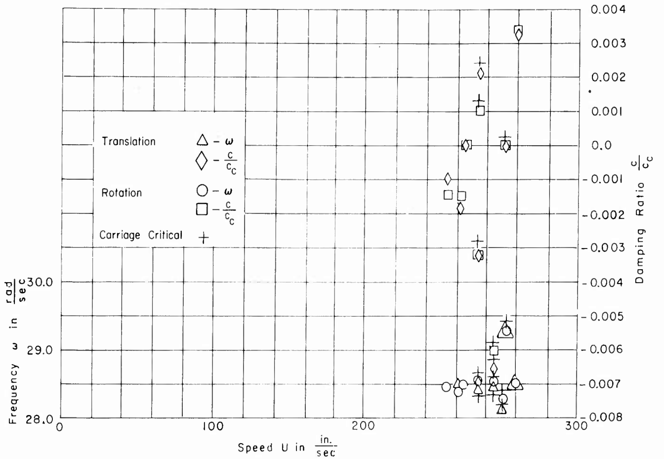
Figure 7f - Configuration B, S_{\alpha} = 2.49 \text{ lb-sec}^2
