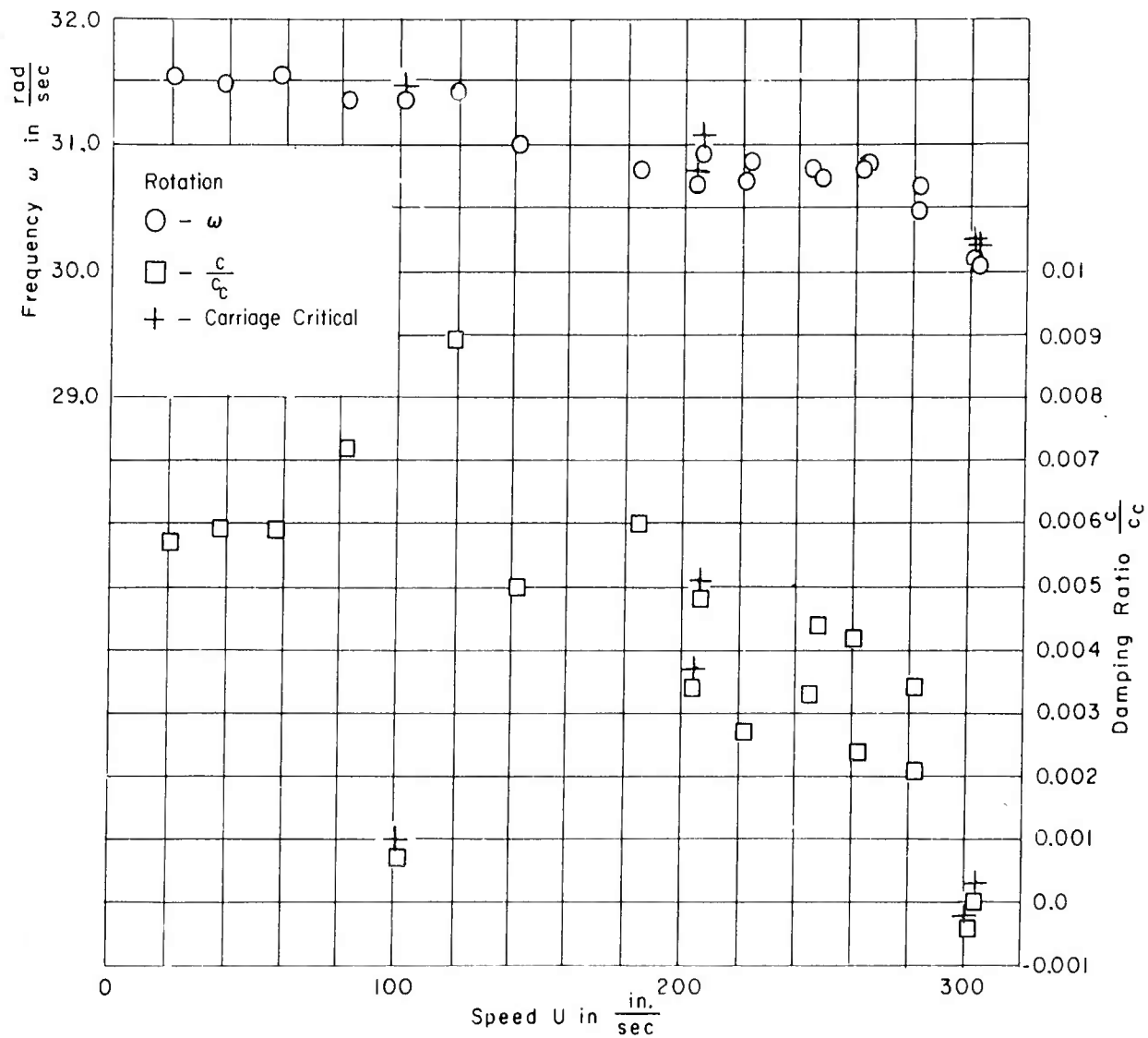
Figure 7a - Configuration A, S_{\alpha} = 2.26 \text{ lb-sec}^2 , Rotation
