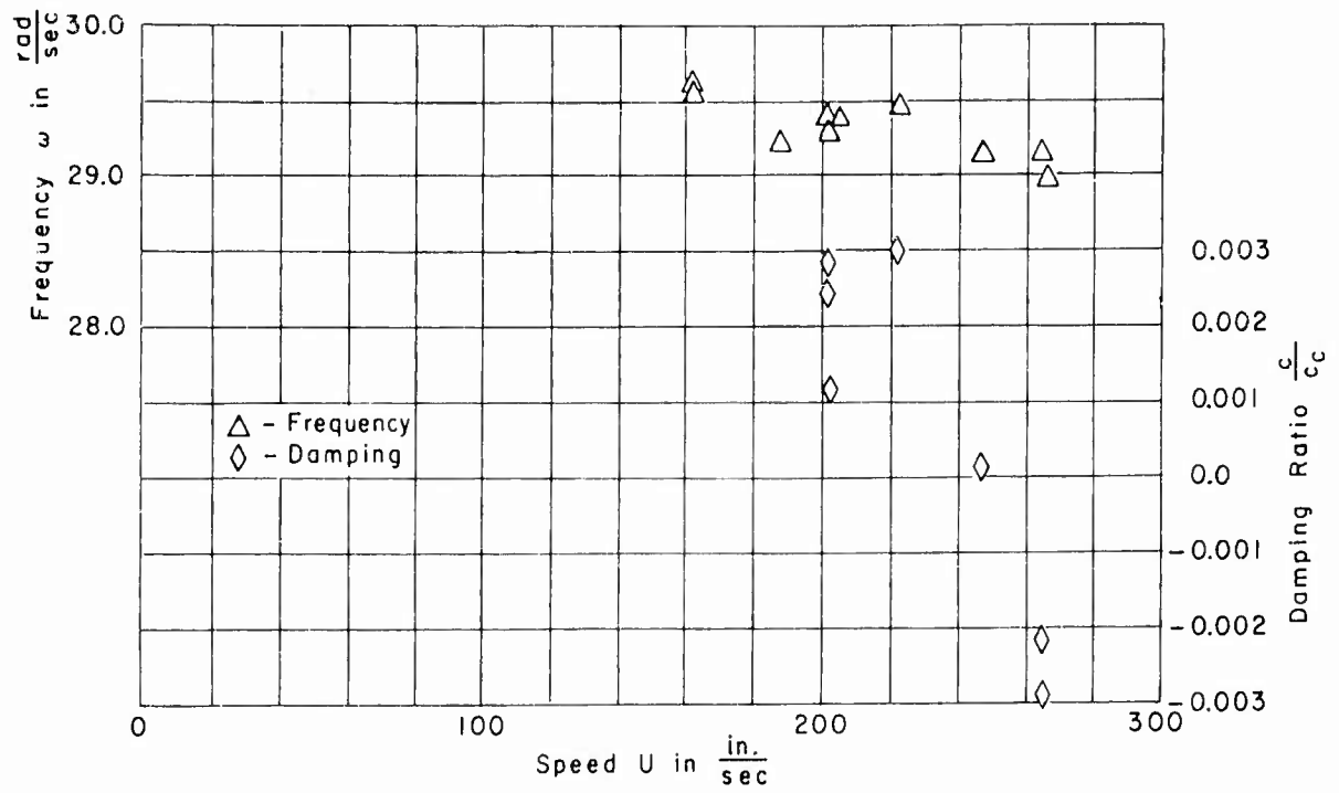
Figure 7m - Configuration B, S_{\alpha} = 2.86 \text{ lb-sec}^2 , Translation
