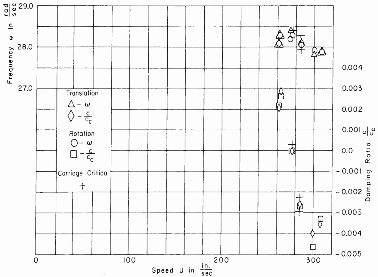
Figure 7v - Configuration D, S_\alpha = 2.93 \text{ lb-sec}^2
