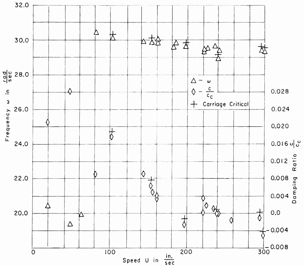
Figure 7p - Configuration B, S_{\alpha} = 2.93 \text{ lb-sec}^2 , Translation
