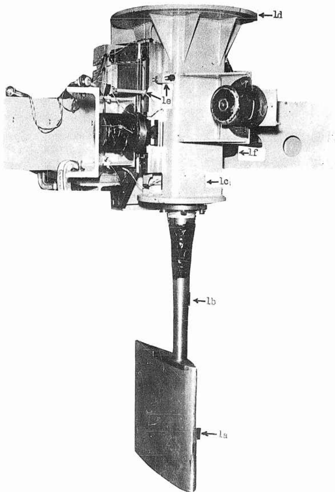
Figure 1 - TMB Flutter Apparatus
