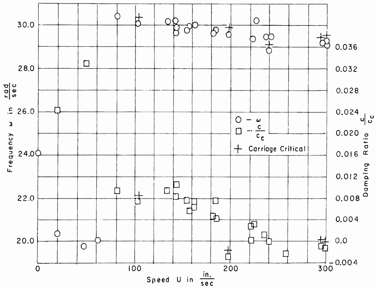
Figure 7n - Configuration B, S_{\alpha} = 2.93 \text{ lb-sec}^2 , Rotation
