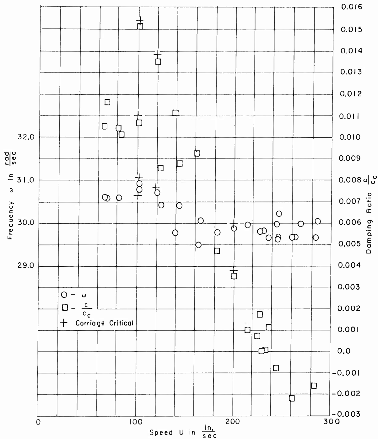
Figure 7q - Configuration B, S_{\alpha} = 3.94 \text{ lb-sec}^2 , Rotation
