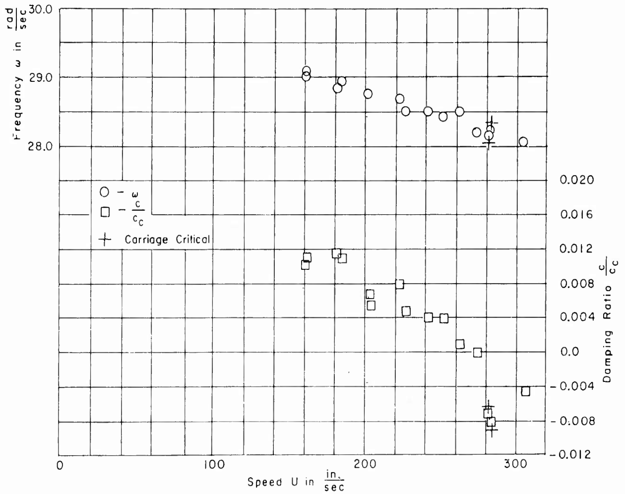
Figure 7w - Configuration D, S_{\alpha}=3.04 \text{ lb-sec}^2 , Rotation
