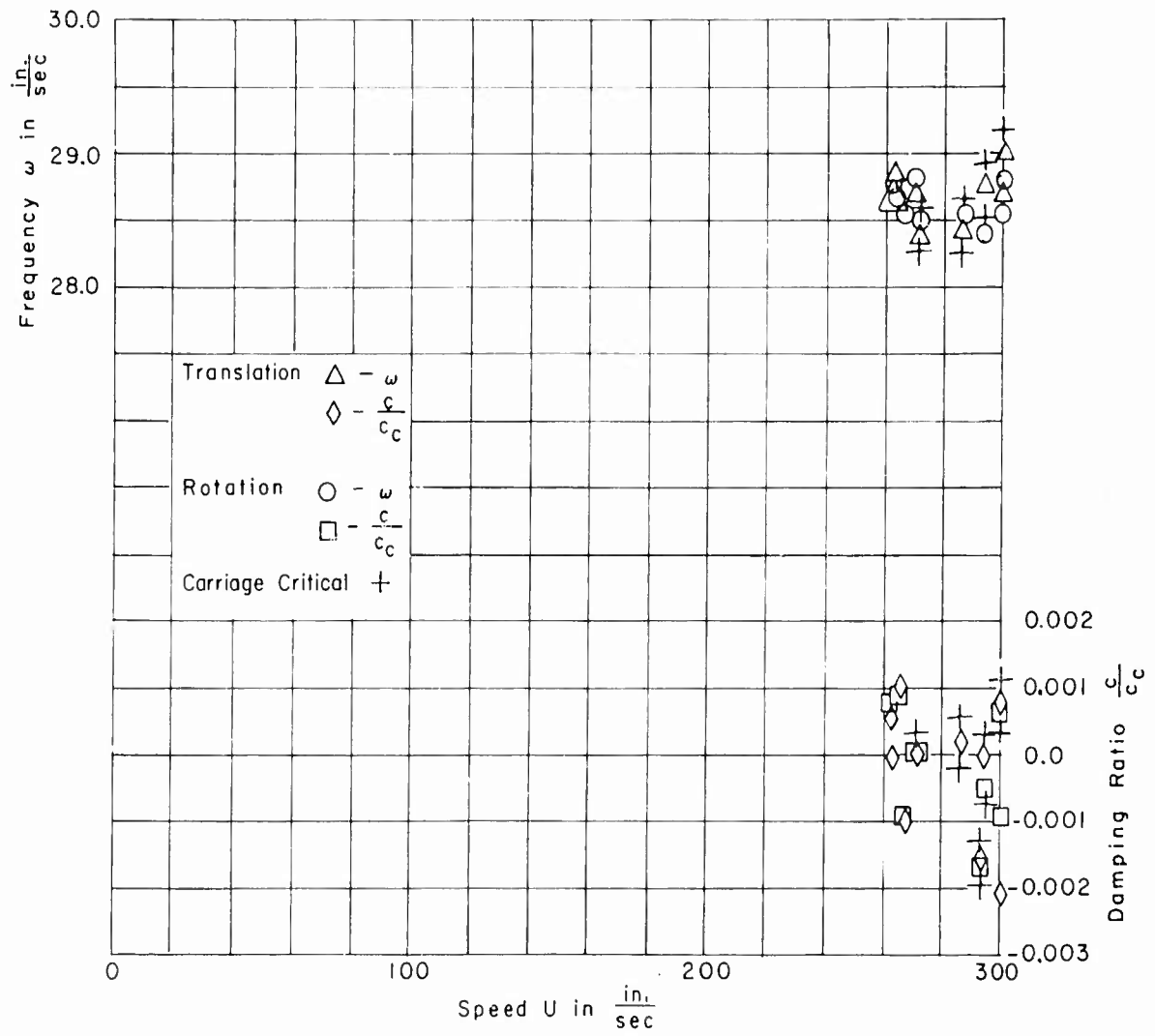
Figure 7g - Configuration B, S_{\alpha} = 2.54 \text{ lb-sec}^2
