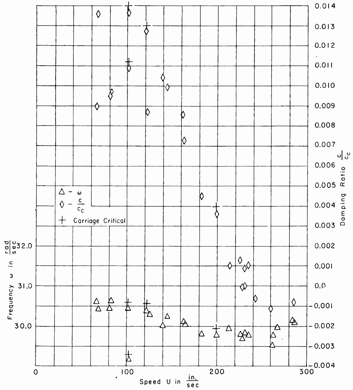
Figure 7r - Configuration B, S_{\alpha} = 3.04 \text{ lb-sec}^2 , Translation
