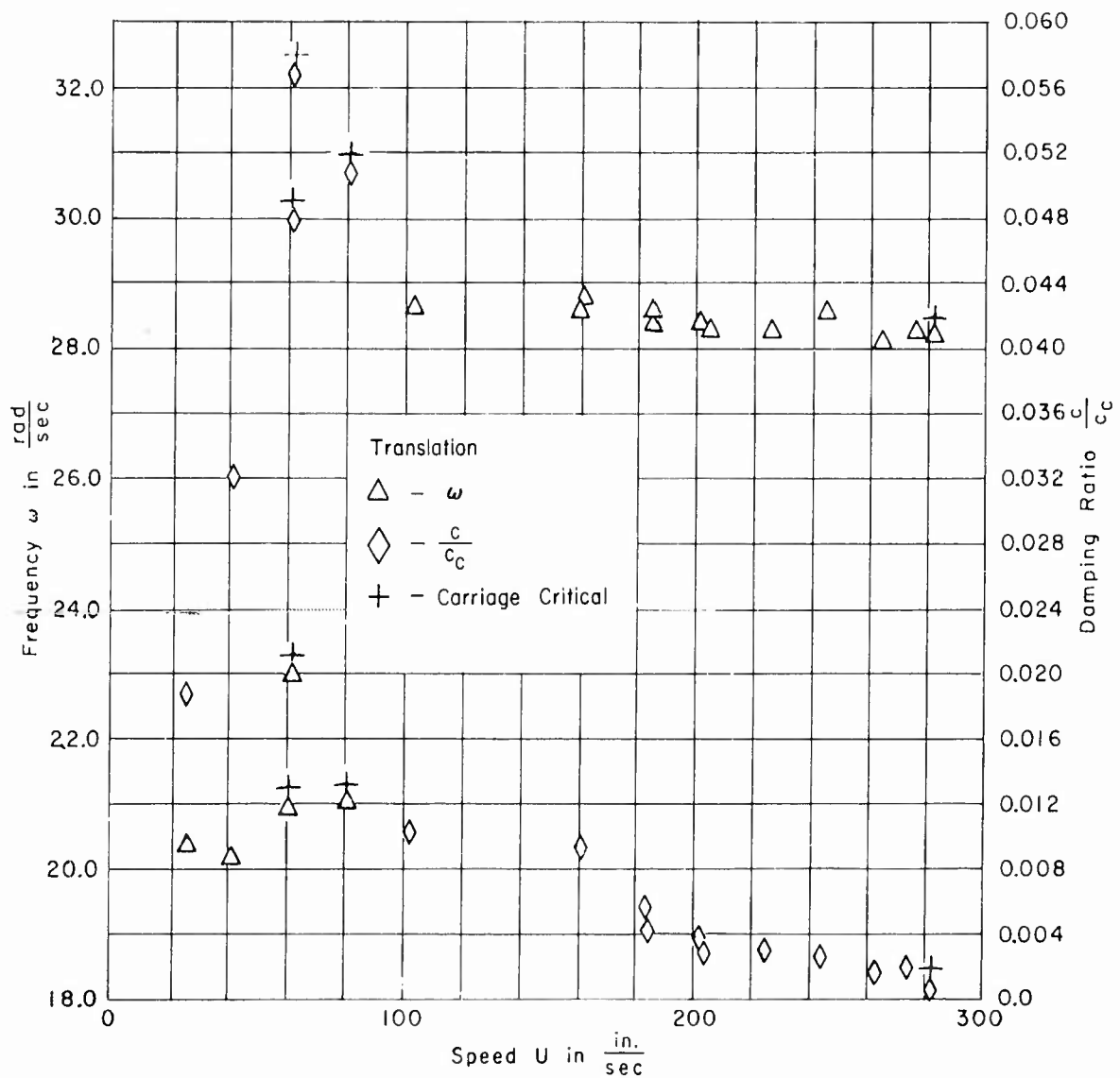
Figure 7e - Configuration B, S_{\alpha} = 2.25 \text{ lb-sec}^2 , Translation
