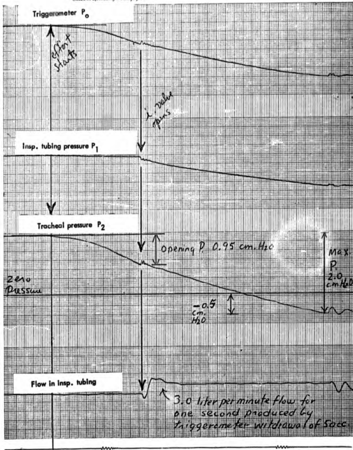
Figure 28. Pressure and Flow Curves obtained from Analogue shown in Figure 27. BIRD Ventilator turned off. Patient's "effort" opens inspiratory Sierra check valve and develops 2 cm. pressure change.
