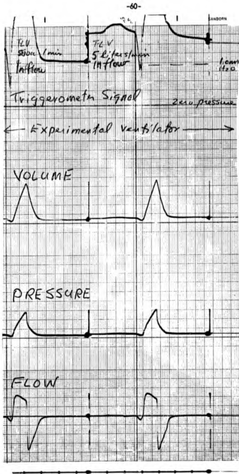
Figure 33. Performance of Experimental Ventilator in Lung Model of Figure 26.
