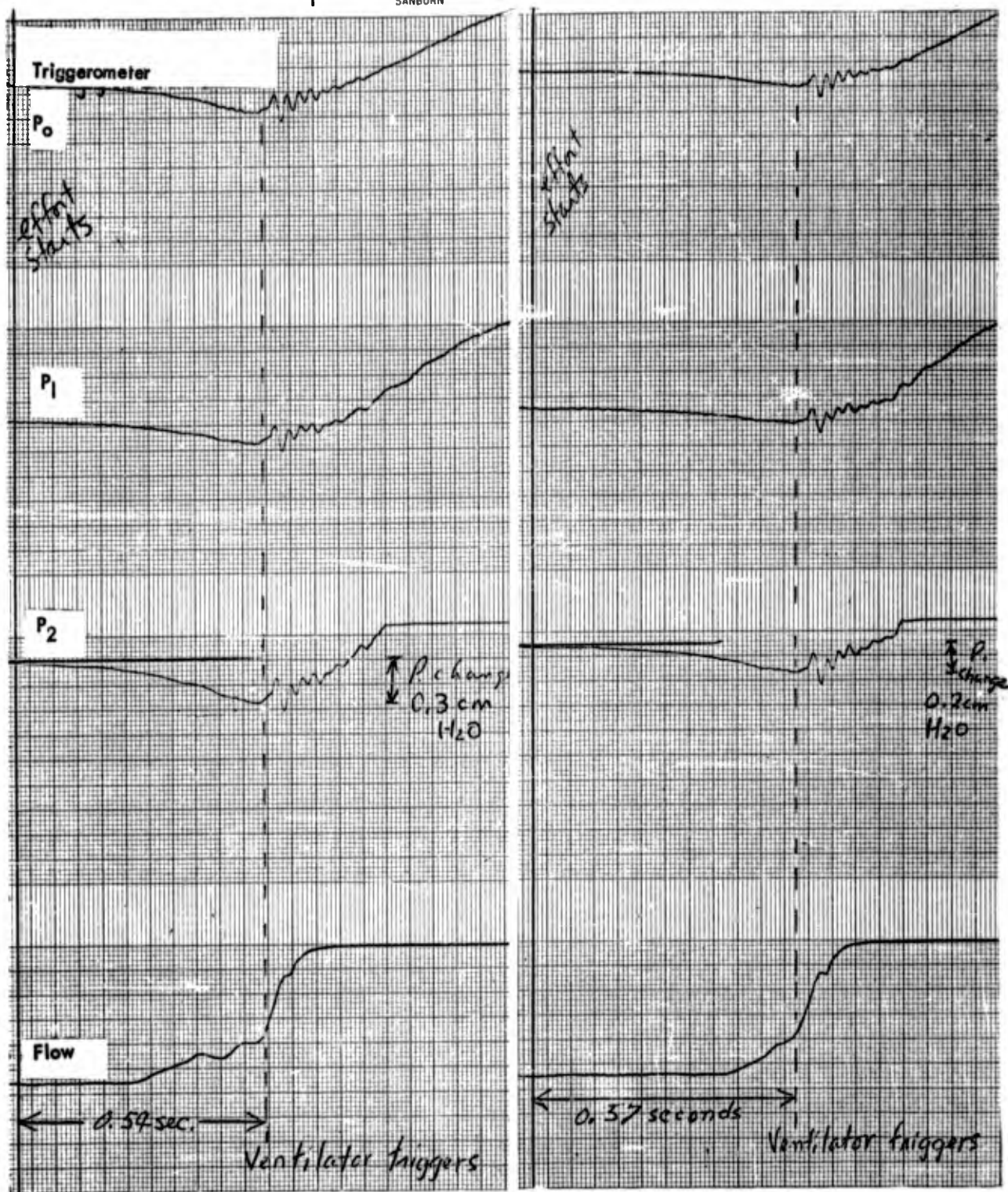
Figure 30. BKD, Mark 5. 500 cc. and 5 liters gas inflow, Ohio check valves at Absorber. Comparable performance.
