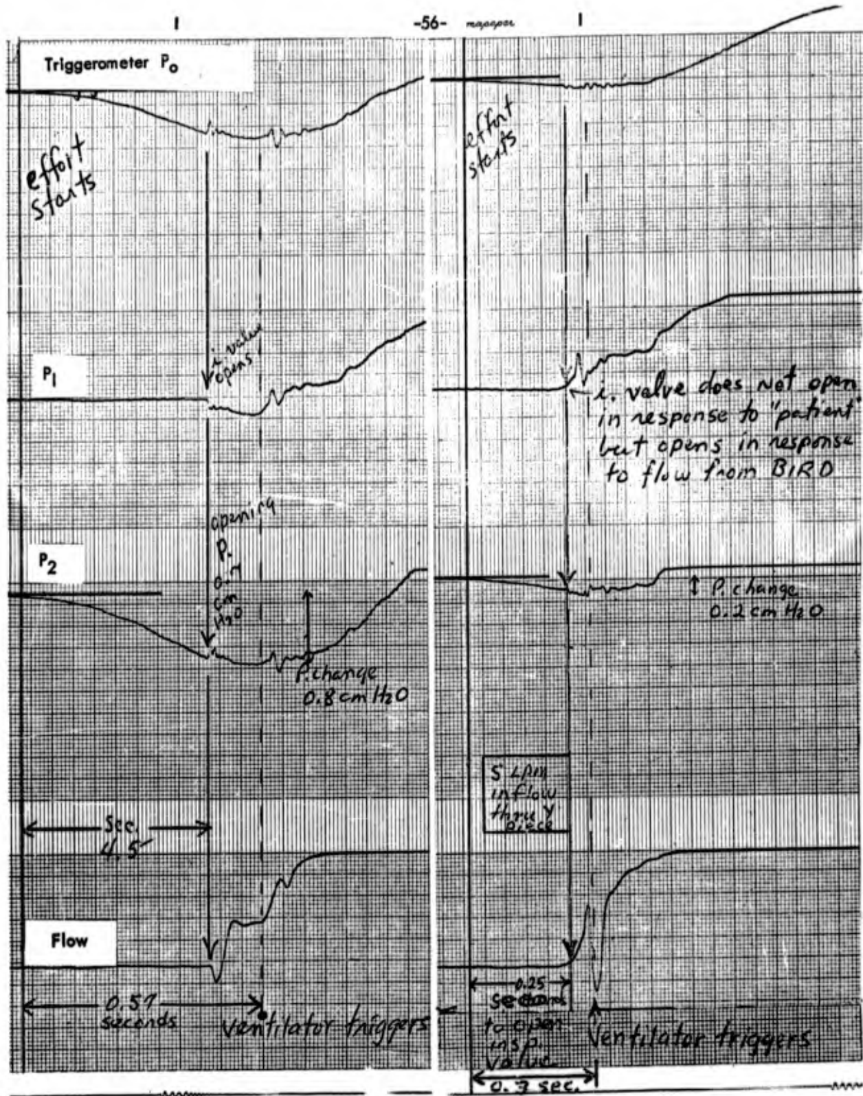
Figure 29. BIRD, Mark 4. 500 cc. and 5 liters gas inflow. Sierra check valves at tracheal tube improve semi-closed system.
