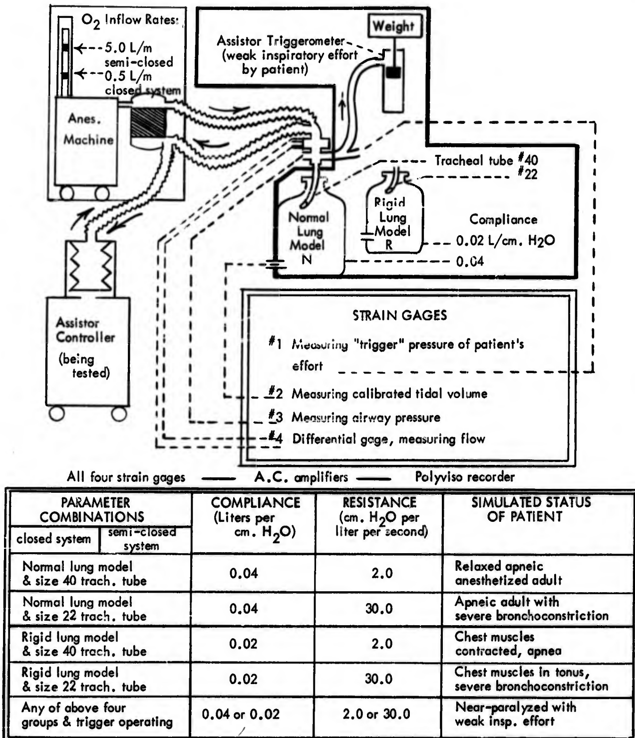
Figure 26. DIAGRAM OF CIRCUITS AND MEASUREMENTS FOR RECORDING OBJECTIVE PERFORMANCE OF ASSISTOR-CONTROLLERS
