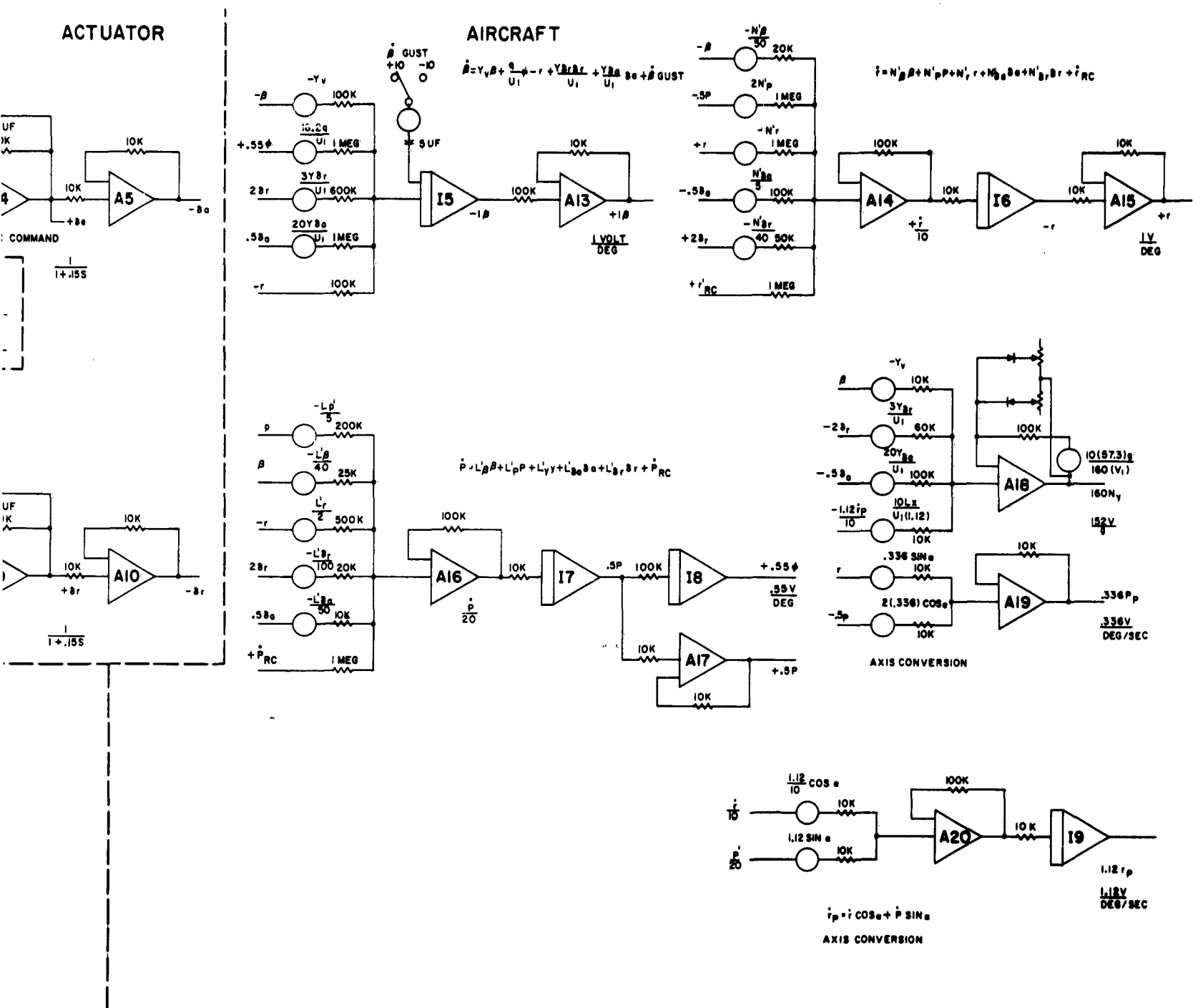
Figure 3. Lateral Axis Simulation
