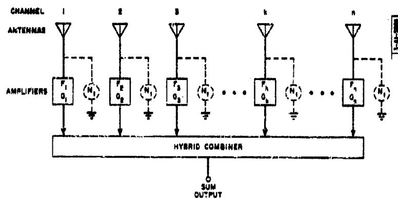
Fig. 2-54. Block diagram of phased array receiver.
