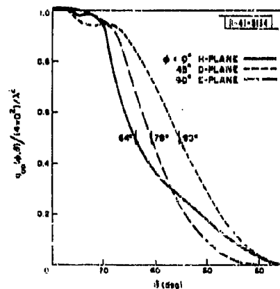
Fig. 3-40. Normalized gain function, g_{00}(\phi, 0)/(4\pi D^2/\lambda^2) , for center element of 9 X 7 array for element spacing D = 0.7\lambda and element height above ground plane s = 0.125\lambda . Also indicated is the included angle over which the array may be scanned in each plane with less than 3-db loss in gain.
