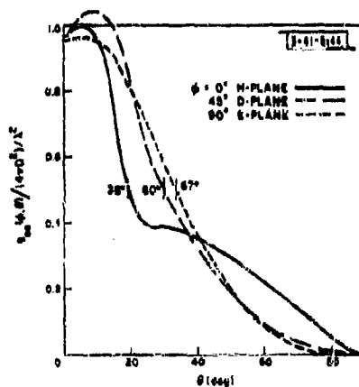
Fig. 3-50. Normalized gain function, g_{00}(\phi, \theta)/(4\pi D^2/\lambda^2) , for center element of 9 \times 7 array for element spacing D = 0.8\lambda and element height above ground plane s = 0.250\lambda . Also indicated is the included angle over which the array may be scanned in each plane with less than 3-dB loss in gain.
