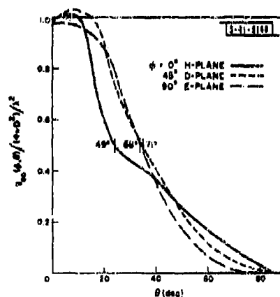
Fig. 3-46. Normalized gain function, g_0(\theta, 0)/(4\pi D^2/\lambda^2) , for center element of 9 X 7 array for element spacing D = 0.8\lambda and element height above ground plane s = 0.125\lambda . Also indicated is the included angle over which the array may be scanned in each plane with less than 3-dB loss in gain.
