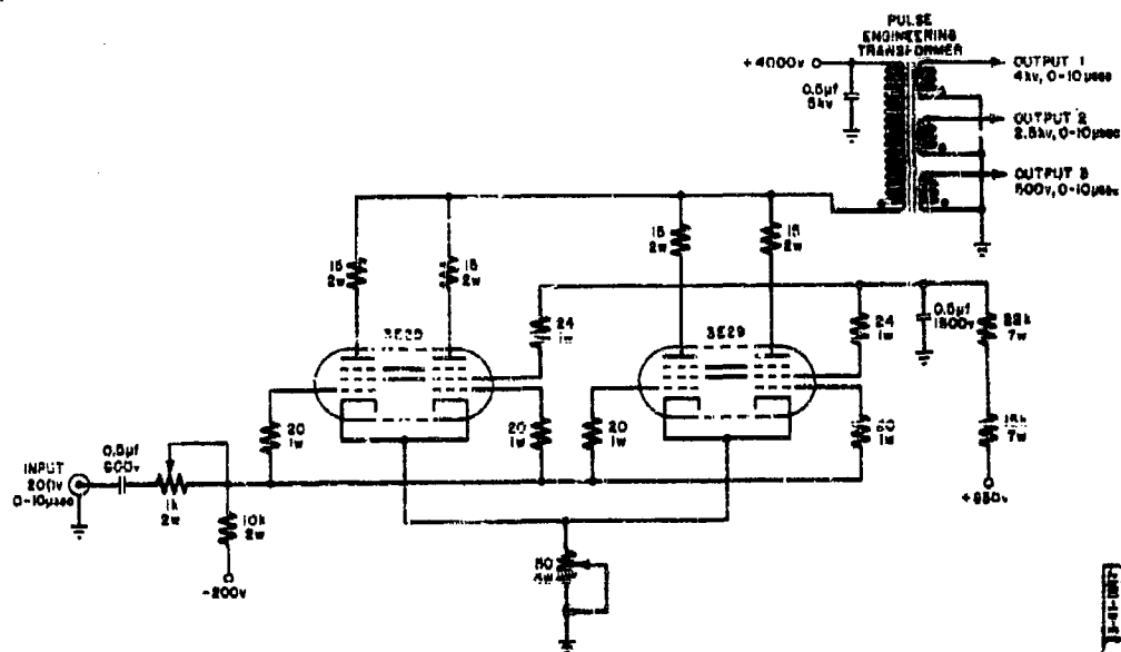
Fig. 2-86. Schematic diagram of pulse modulator.
