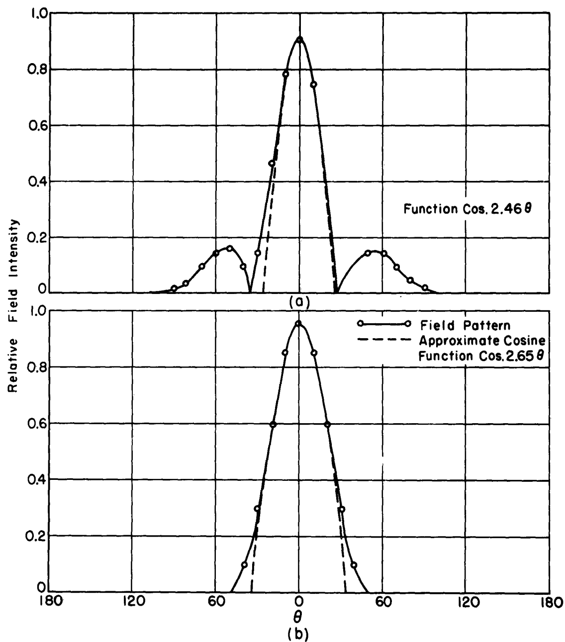
Fig. 15. Field pattern of No. 6 horn. a. E-field. b. H-field.
