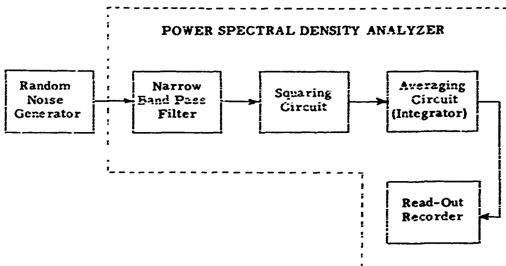
Figure 8.4 Equipment for Testing Power Spectra Measurement Accuracy
