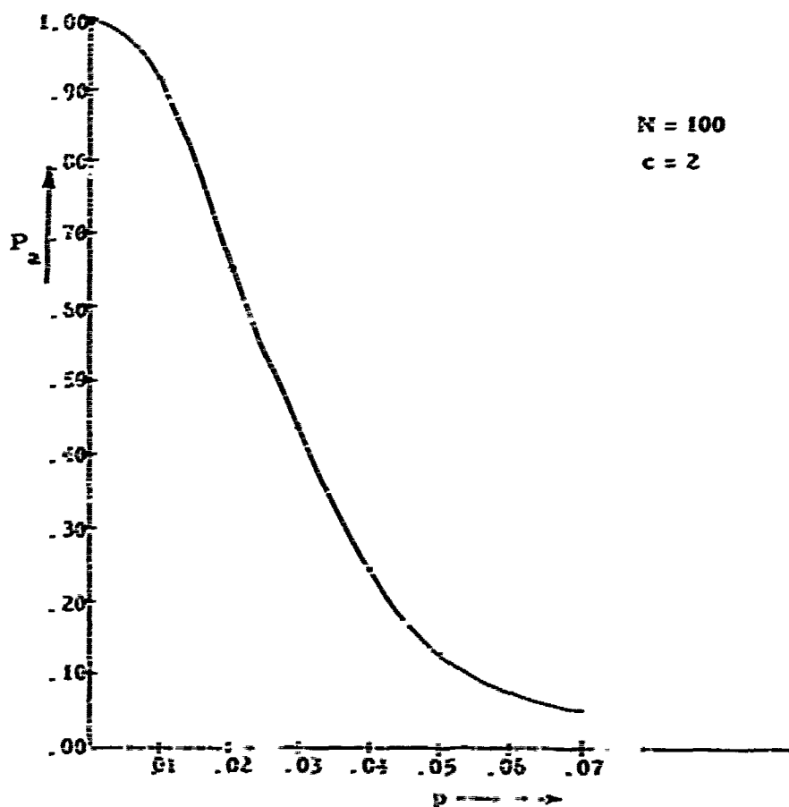
Figure 5.2. O.C. Curve for Single Sampling Plan
