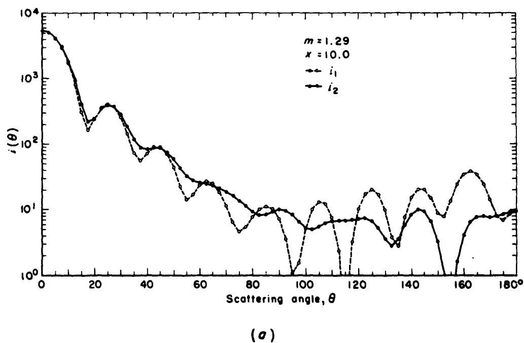
FIG. 9—The logarithm of the intensities i_1 (dashed line) and i_2 (full line) for spheres with x = 10 , plotted at intervals of 2^\circ.5 in \theta . The curves for m = 1.29 and 1.29 - 0.4720i are shown separately in (a) and (b), respectively.
