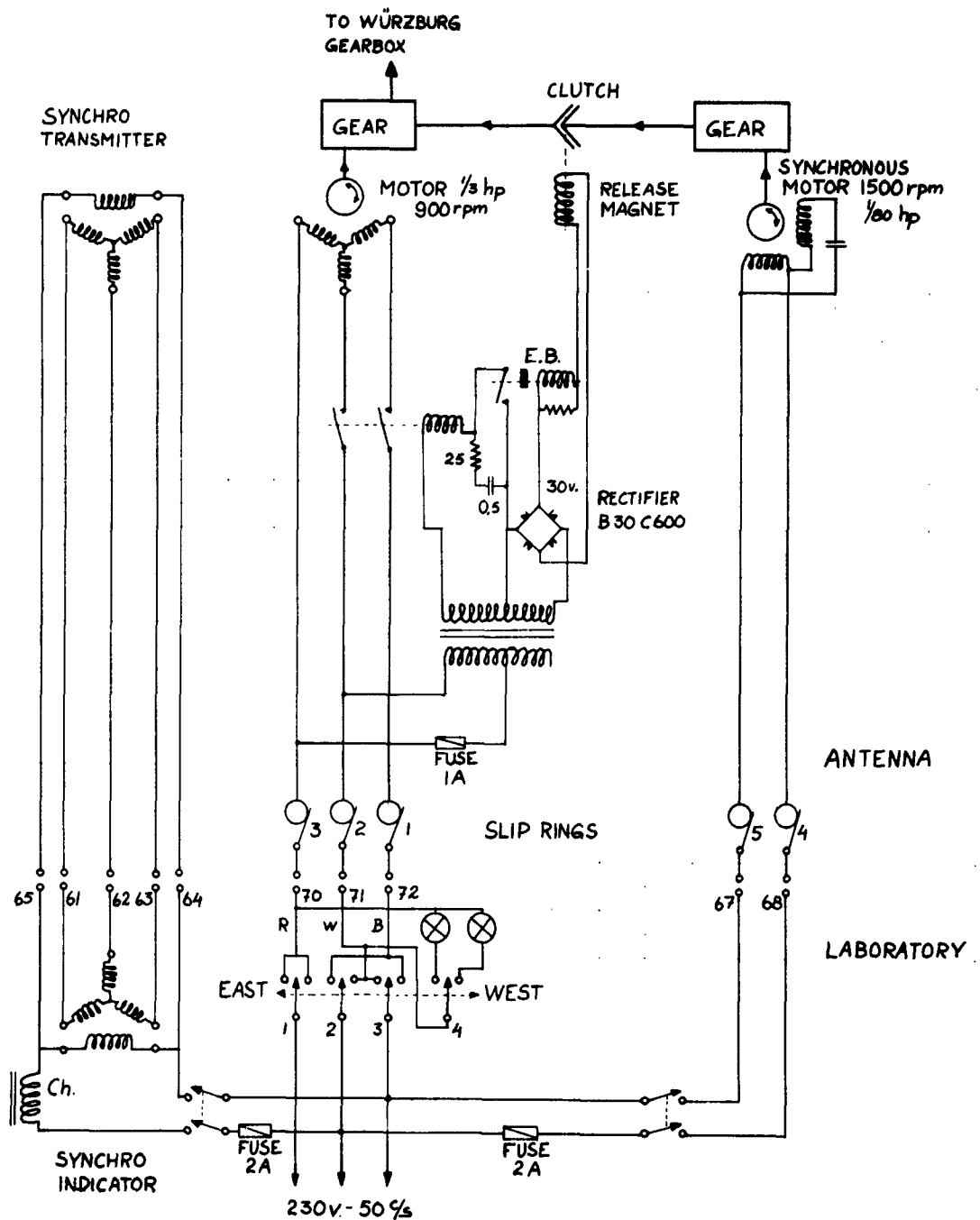
Fig. 3. Hour angle driving mechanism.
