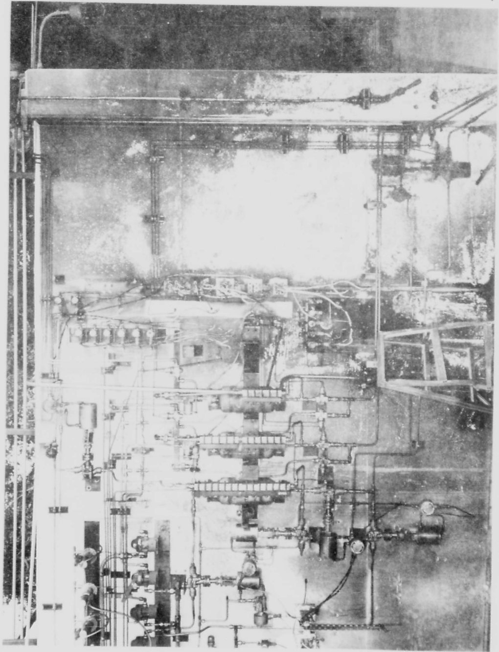
Figure 10. Hazard Classification Test Stand Following Pentaborane System Failure
