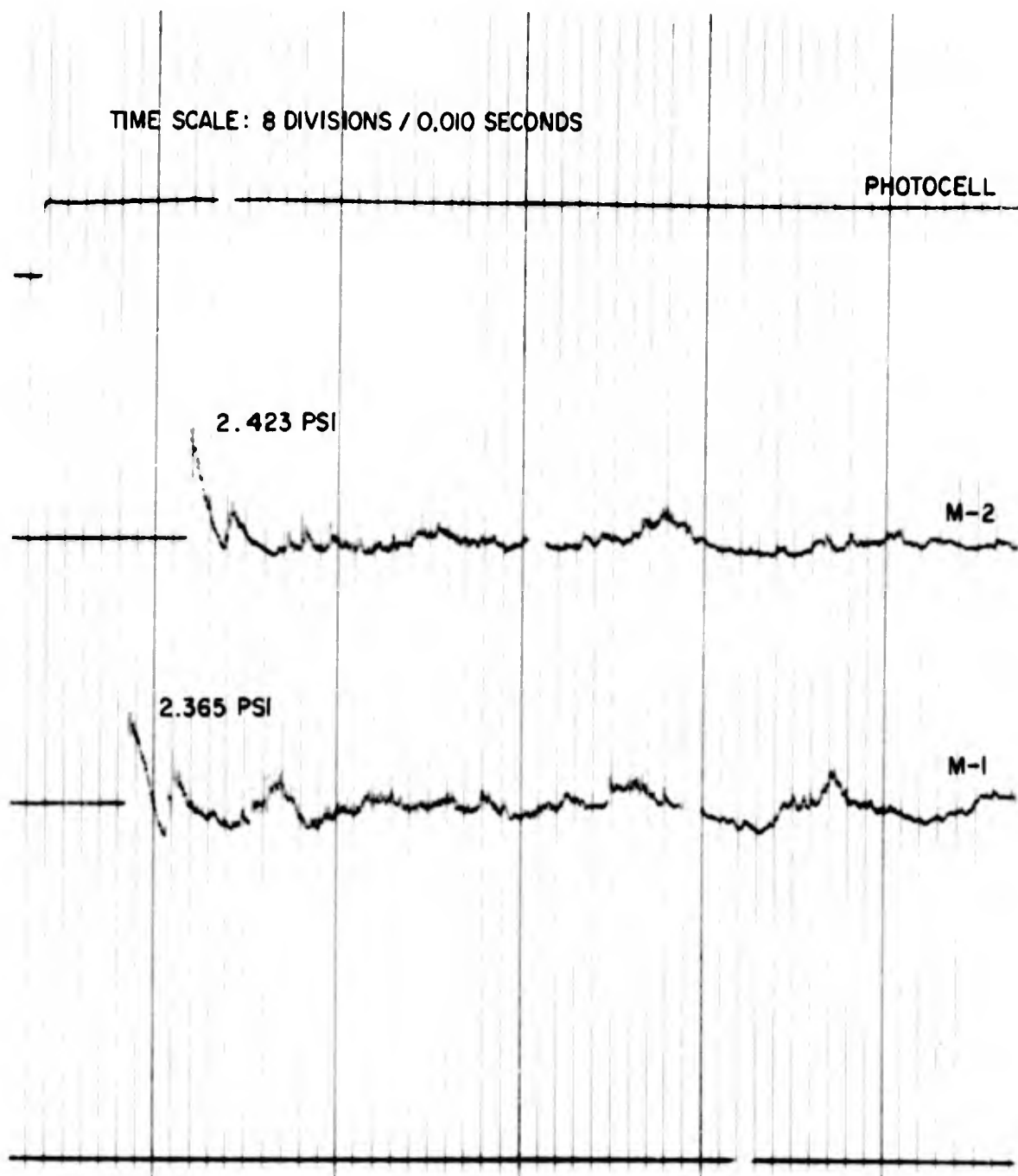
Figure 25. Overpressure Resulting from a Simultaneous Spill of Hydrazine and Pentaborane on Asphalt
