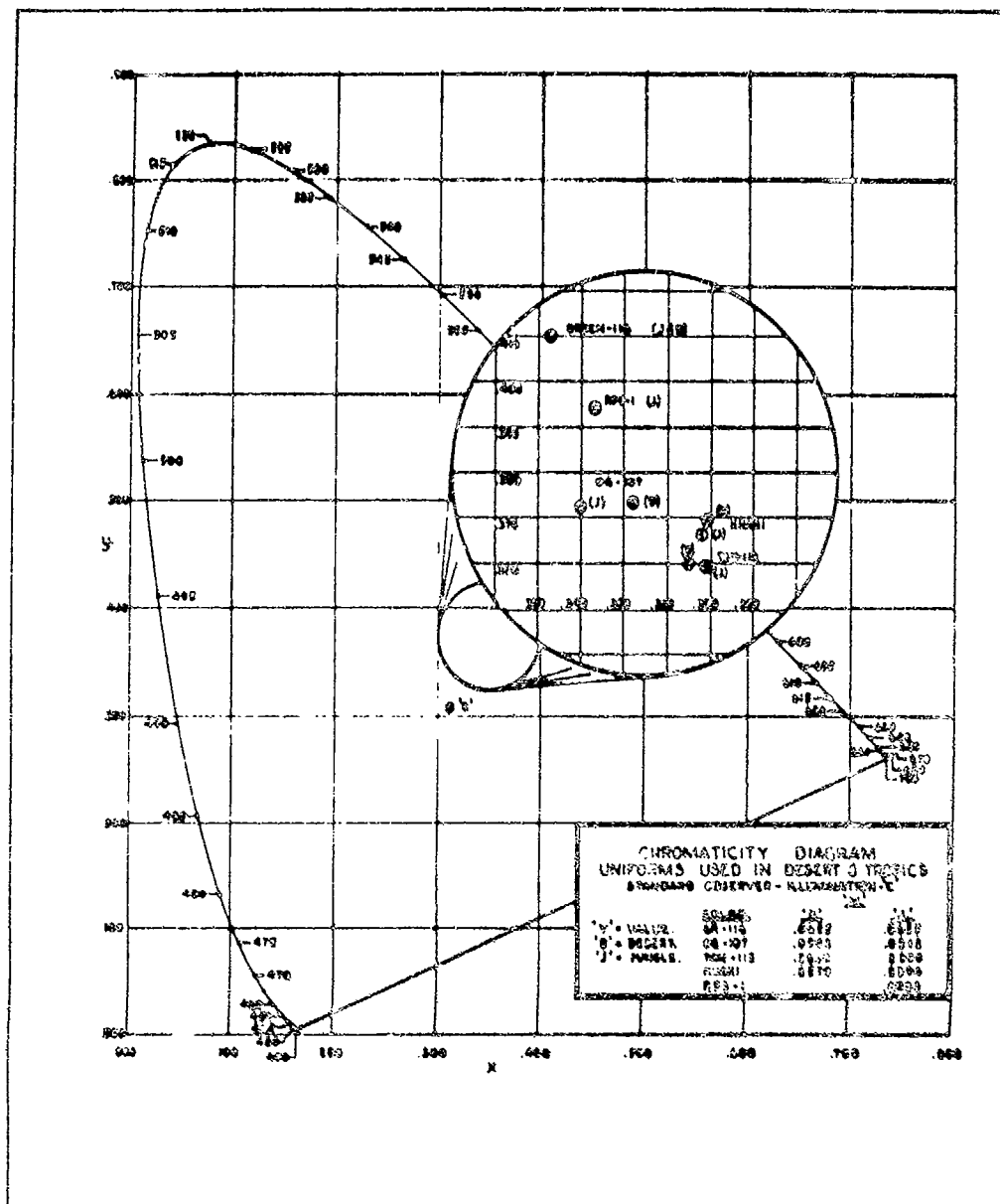
Fig. 62. Chromaticity diagram of uniforms used in desert and tropics.
