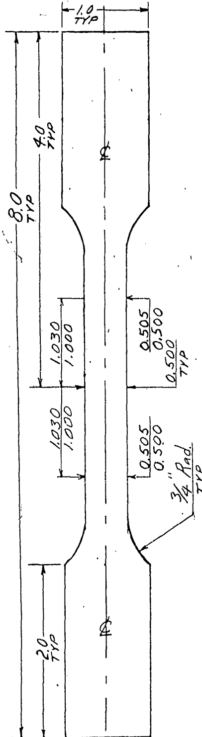
Standard Tensile Specimen
