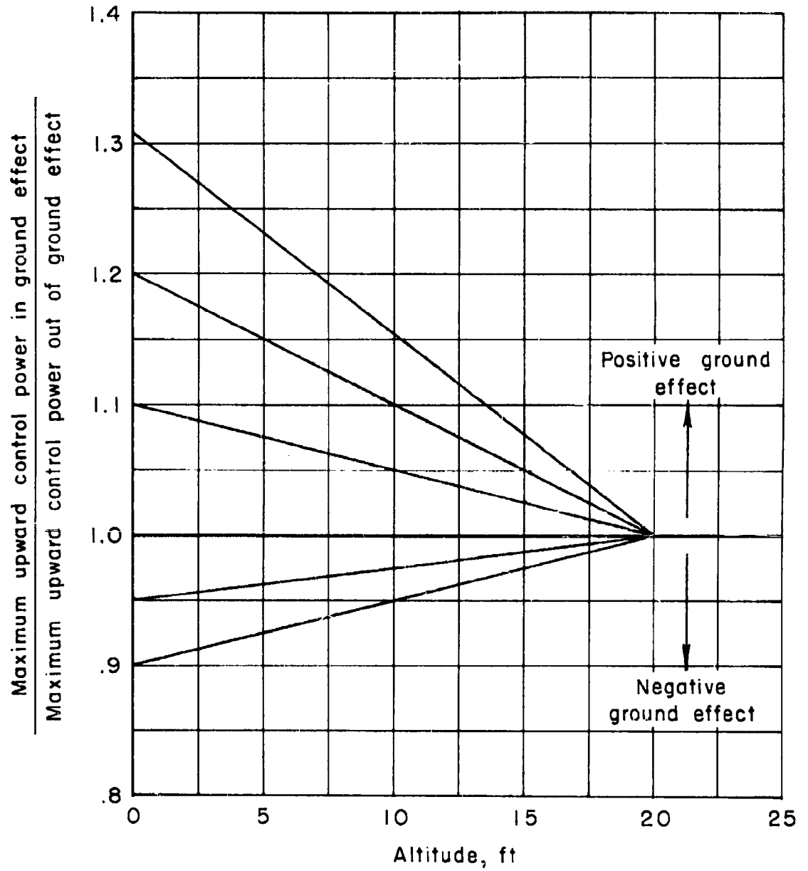
Figure 4.- Five variations in levels of ground effect used.
