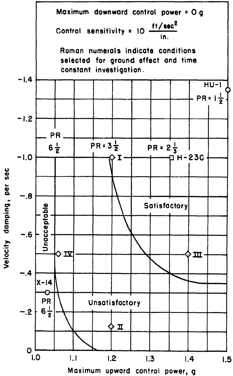
Figure 6.- Maximum control power boundaries out of ground effect and with control system time constant of zero.
