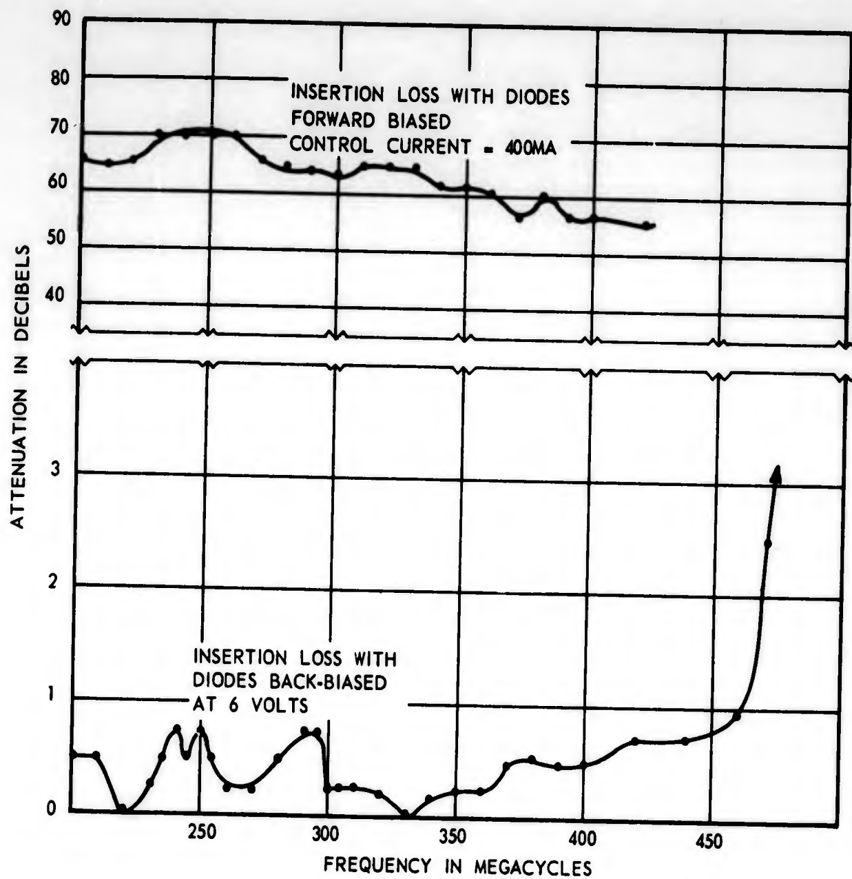
Figure 6. Switch Insertion Loss Characteristics.
