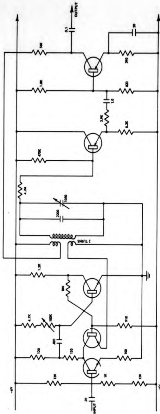
Figure 13. Locked Oscillator.
