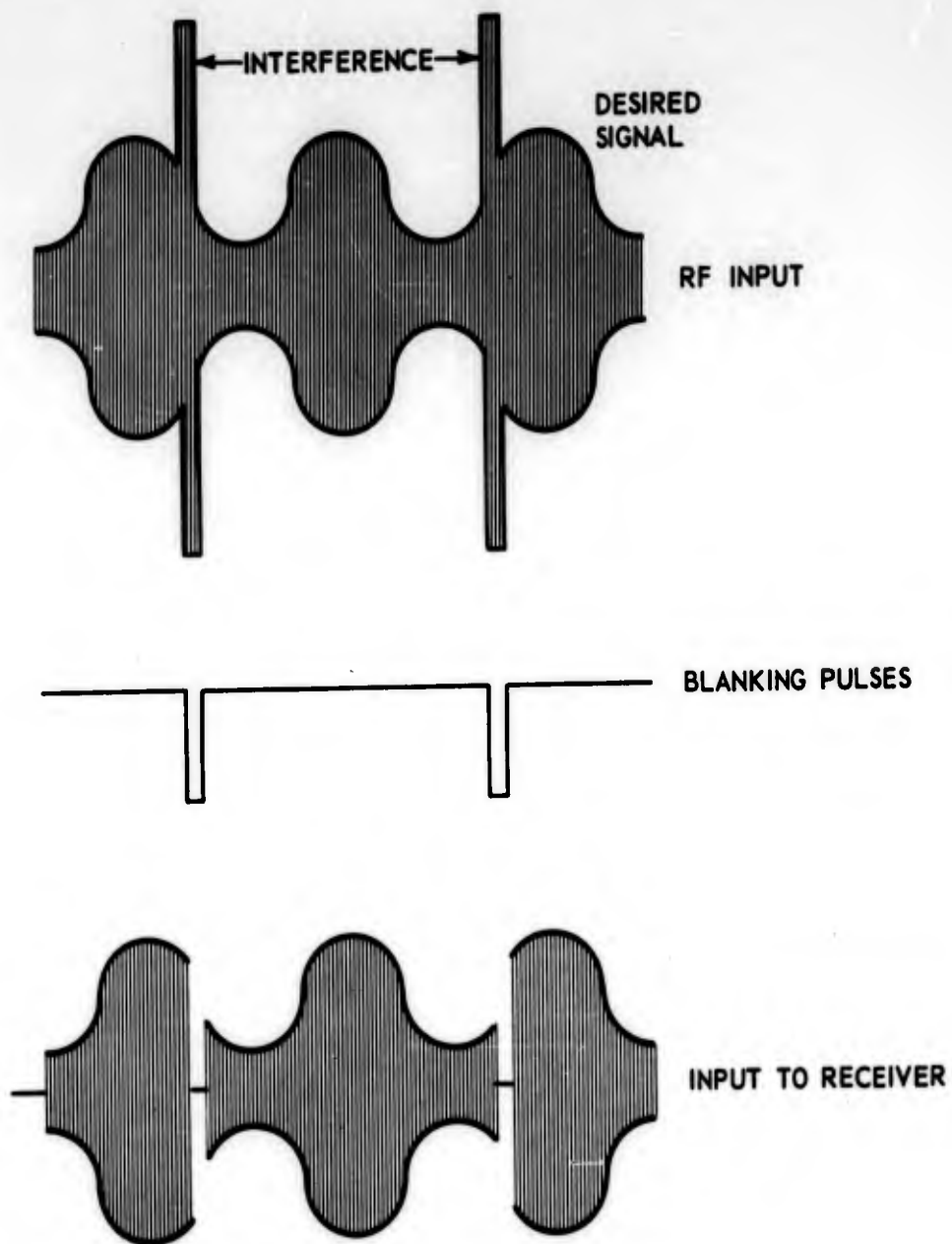
Figure 2. Blanking Waveforms.
