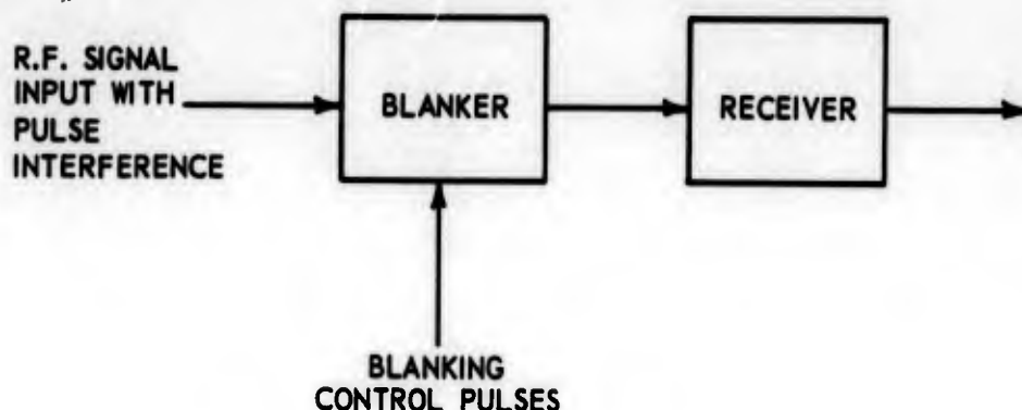
Figure 1. Interference Blanking
