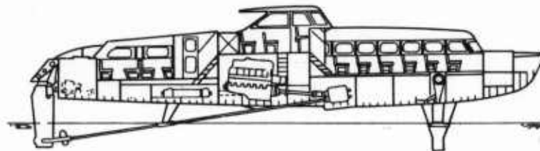
Exhibit 12. Sectional Drawing of the Supramar PT 20.
