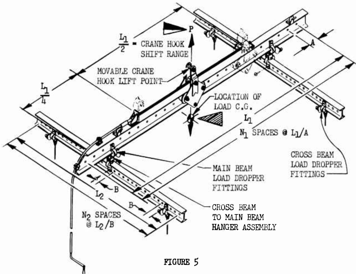
HOISTING SYSTEM
