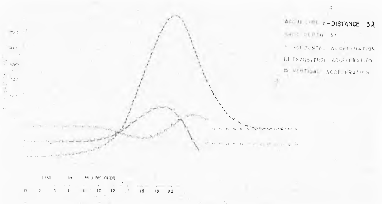
FIGURE 37- ACCELERATIONS vs. TIMES IN CLAY
