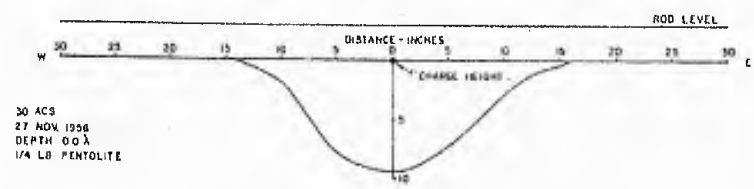
FIGURE 24. TYPICAL TRUE CRATER PROFILES IN SAND FOR SHOTS FROM 0 TO 1.5 SHOT DEPTH (SCALE RADII)
