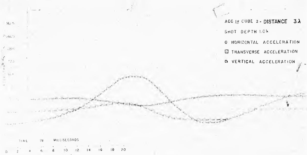
FIGURE 39-ACCELERATIONS vs. TIMES IN CLAY
