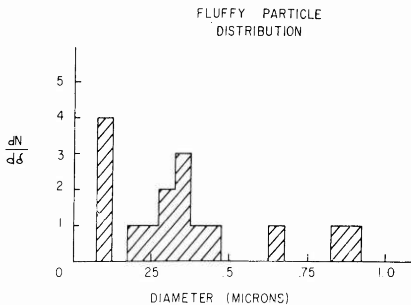
Fig. 17. Size distribution of irregular micrometeorites (0.1 to 1 micron).
