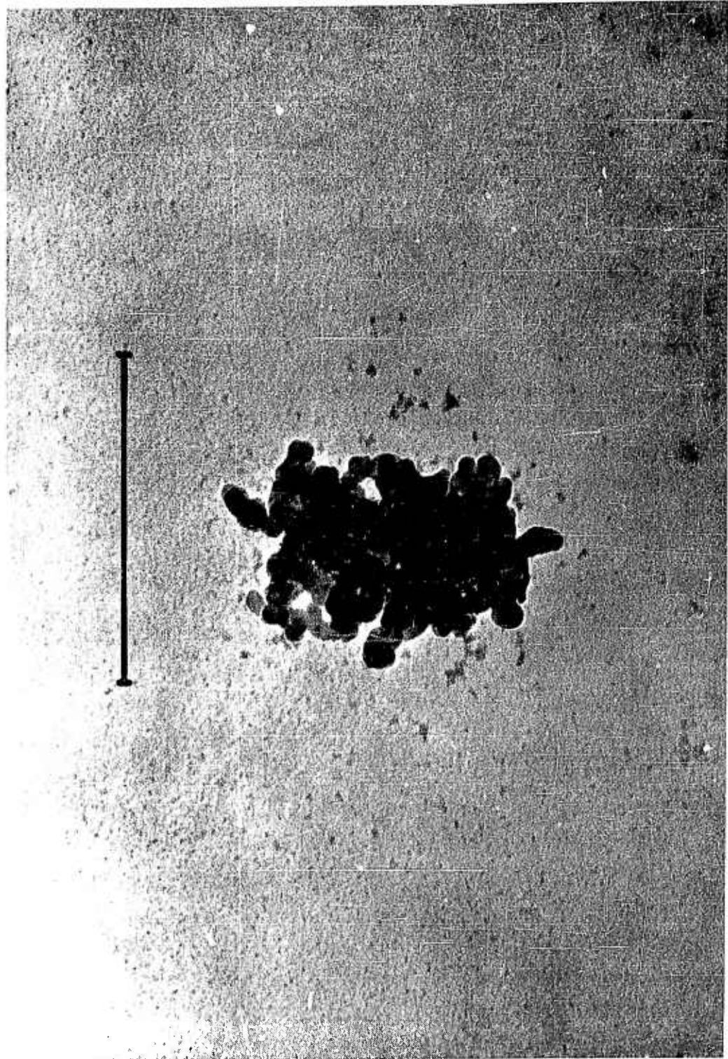
Fig. 11. "Fluffy" particle obtained from U-2 collection (scale = 2.5 micron).
