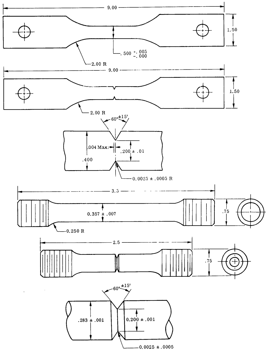
Fig. 1. Tensile specimens for cryogenic testing (all dimensions in inches).
