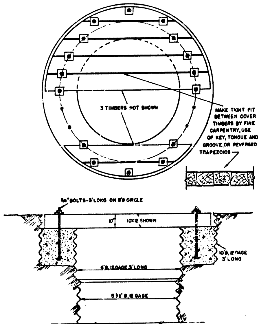
Fig. 40. Concentric ring shaft closure foundation; timber closure illustrated.
