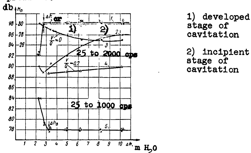
Fig. 5. Change of the general level of vibration of pump No. 1 (RK-2) n = 2500 rpm with different proportions of air and different means for creating rarefaction.
