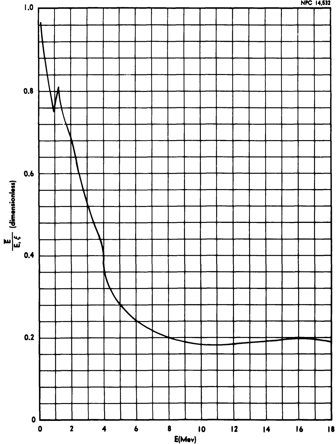
FIGURE B-2. AVERAGE NEUTRON ENERGY LOSS IN IRON
