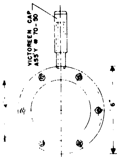
EDWARDS AND KERST IONIZATION CHAMBER
