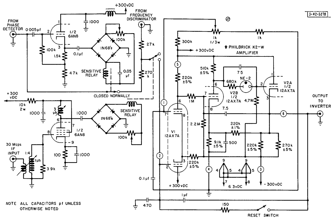
Fig. C-7. Integrator and switching diagram.
