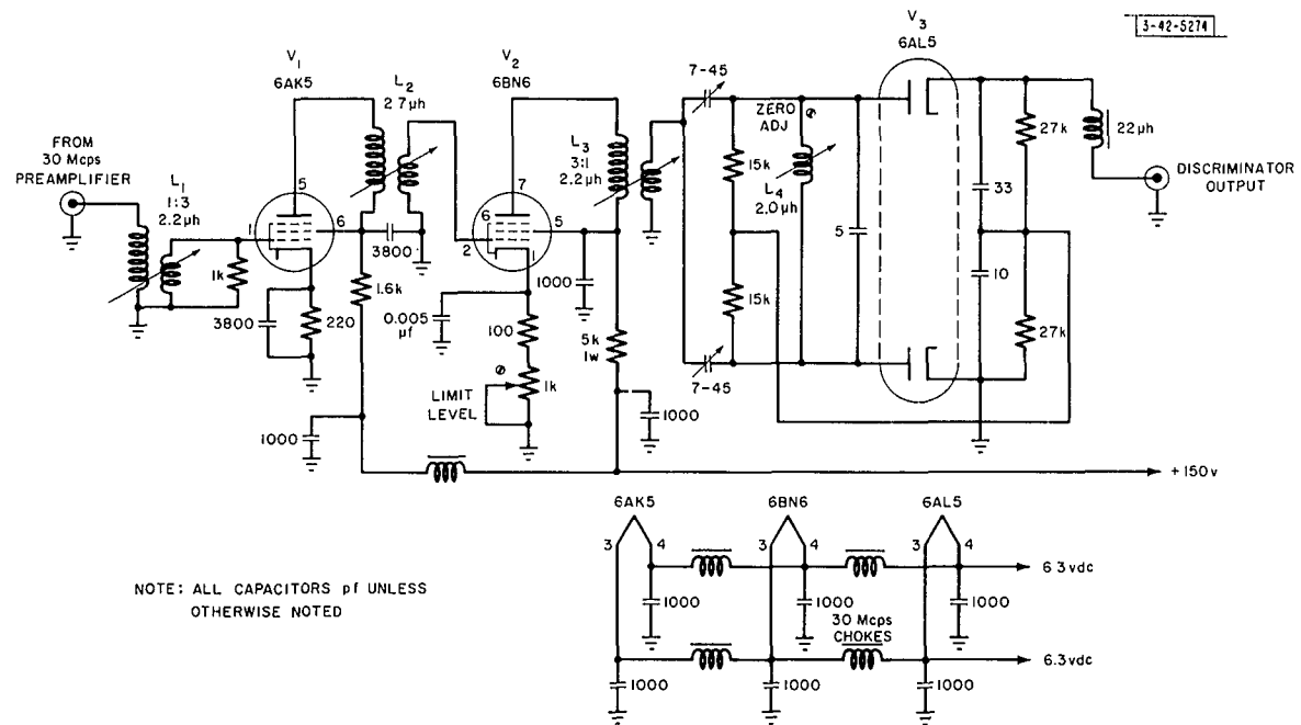
Fig. C-3. 30-Mcps frequency discriminator.
