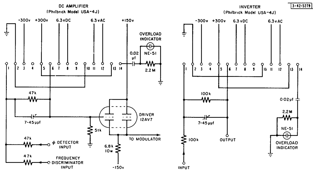
Fig. C-8. DC amplifier, driver and inverter diagrams.
