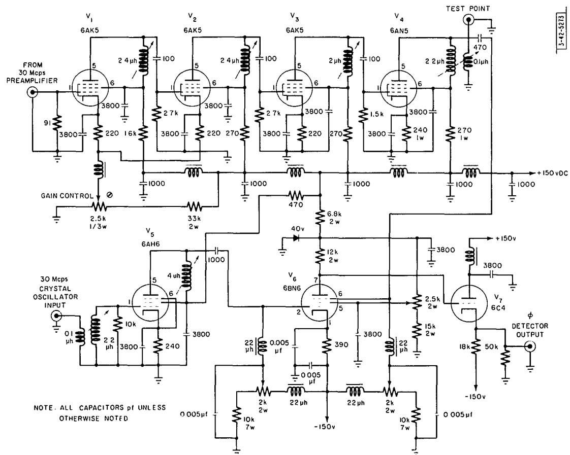
Fig. C-2. 30-Mcps phase detector.
