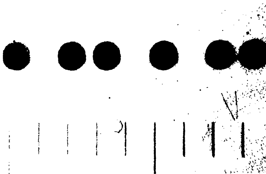
Figure 20. Photomicrograph of a Nine Mil Spot Written on HSP-208.
