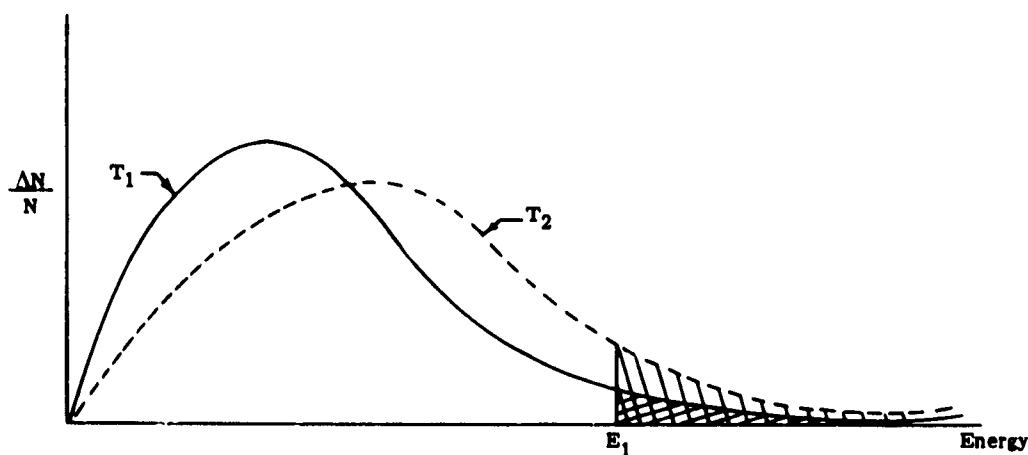
Figure 124. Maxwell-Boltzmann Distribution of Energies.
