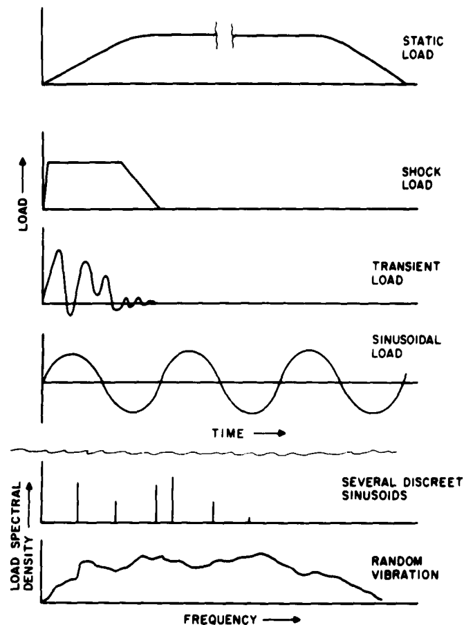
Fig. 1 - Different kinds of load-time functions
