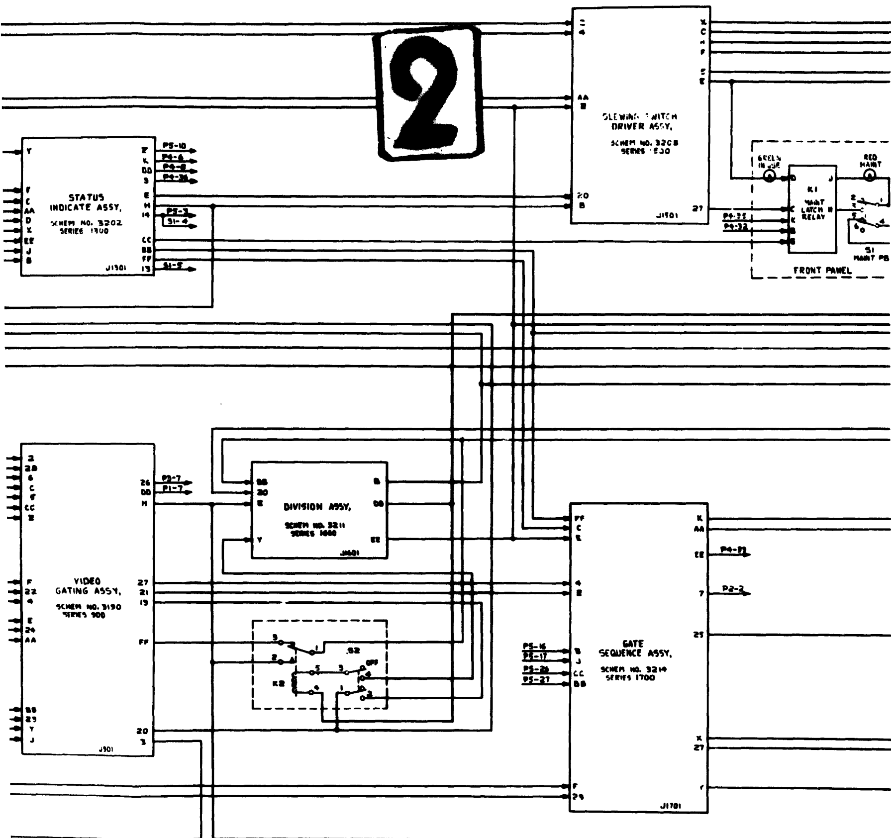
Figure 16. Video Tracker, Block Diagram
