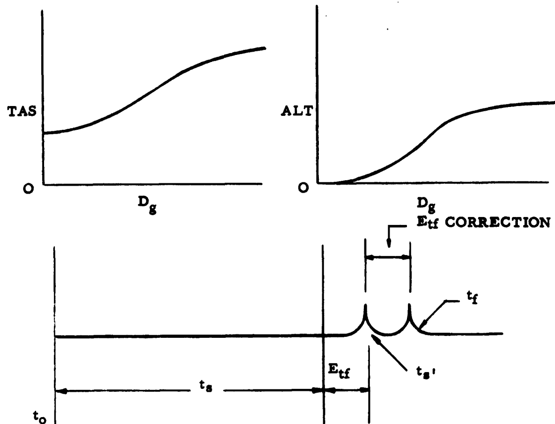
Figure 35. TAS and Altitude Profiles and Derivation of t_s
