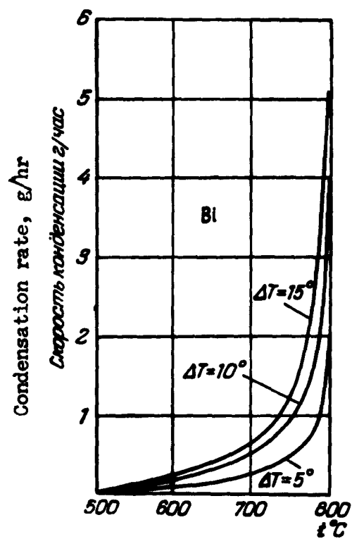
Figure 7. Condensation rate of bismuth vapors on the lid of the bucket depending upon the temperature of the metal and the temperature difference between the metal and the lid, in the absence of a foreign gas in the clearance between the free surface of the metal and the lid.
