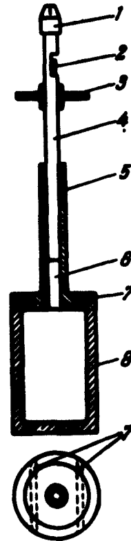
Figure 16. Structure of the suspension system: 1 -- three-jawed chuck for fastening the suspension wire, 2 -- small mirror, 3 -- aluminum disk-radiator, 4 -- porcelain rod (bar), 5 -- graphite lid of crucible, 6 -- free space for excess metal, 7 -- steel bars, for attaching the lid to the crucible, 8 -- graphite crucible.
