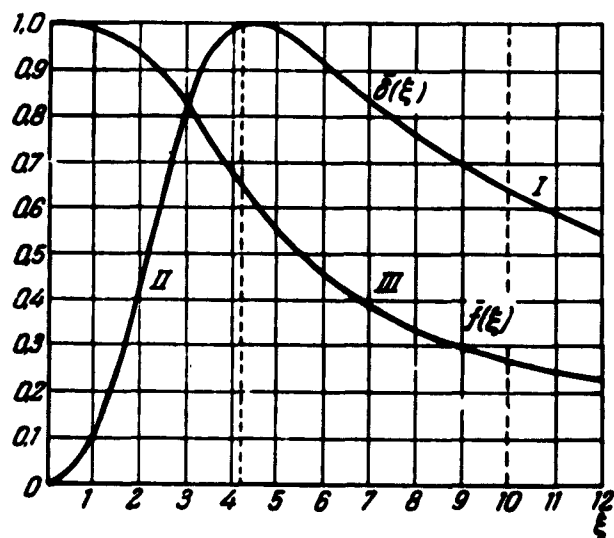
Figure 3. Dependence of the damping decrement \delta(\xi) and function \frac{\tau^2}{\tau_0^2} - 1 = f(\xi) on \xi = R \sqrt{\frac{2\pi}{TV}} . Arbitrary units are plotted along the ordinate axis, and for this reason \bar{\delta}(\xi) and \bar{f}(\xi) differ from their true values by constant factors (multipliers).
