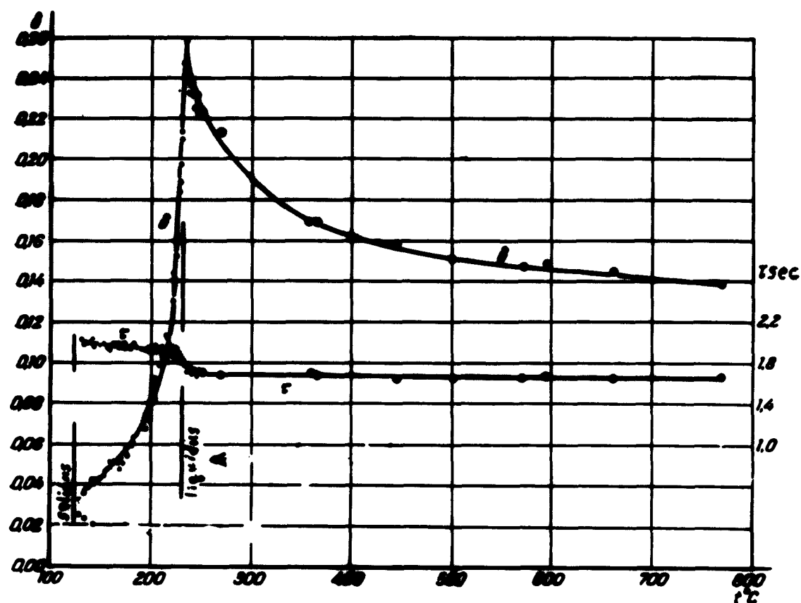
Figure 44. Temperature dependence of the damping decrement and period in a suspension rotary-oscillating viscosimeter, during the study of the viscosity of a 15% Pb + 85% Bi alloy. The solidus and liquidus points (temperatures) are represented by means of vertical lines. The difference in the manner in which points on the curves are represented is due only to their different density of distribution on the line.
