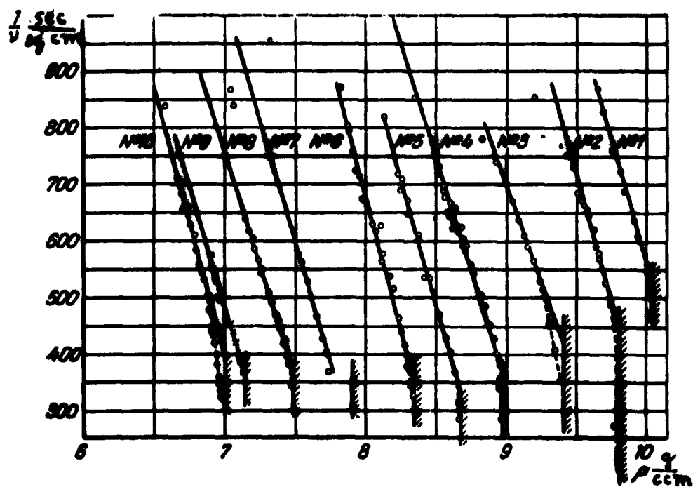
Figure 38. Dependence of \frac{1}{v(p)} for tin-bismuth alloys. No. 1 -- bismuth, No. 10 -- tin. The composition of the alloys is listed in Table 11 (the concentration of tin increases with a growing number of the alloy). Liquidus lines are represented by vertical shaded straight lines.
