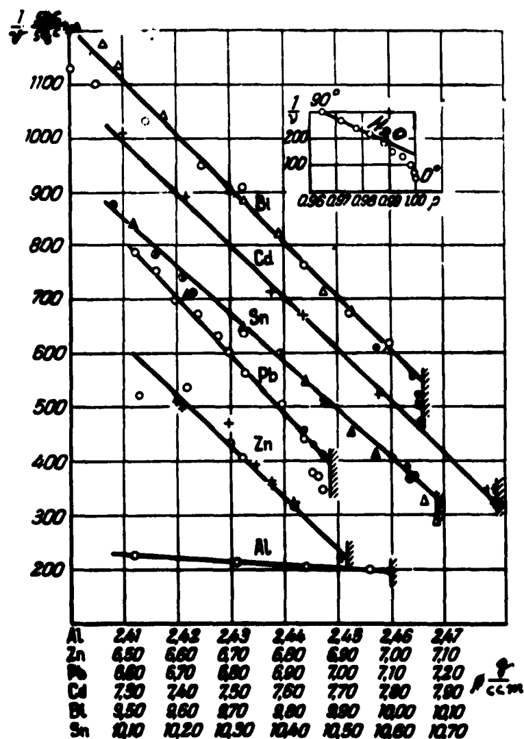
Figure 36. Reciprocal of the kinematic viscosity \frac{1}{\nu} sec/cm 2 as a function of the density.
