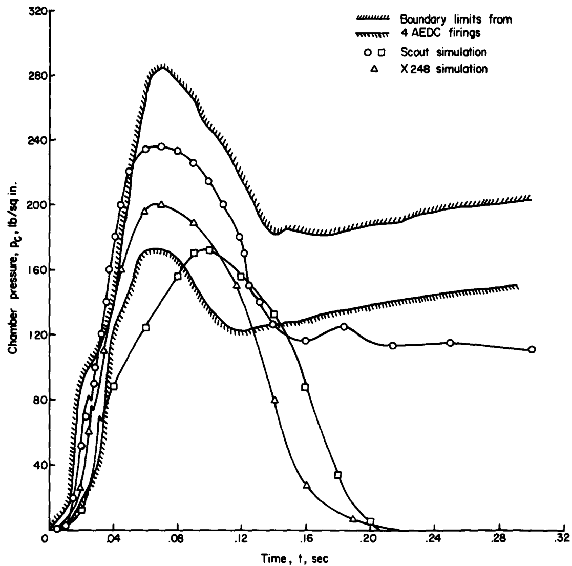
Figure 4.- Motor chamber pressure as a function of time for the test motor and for the flight ABL X248 rocket motor.
