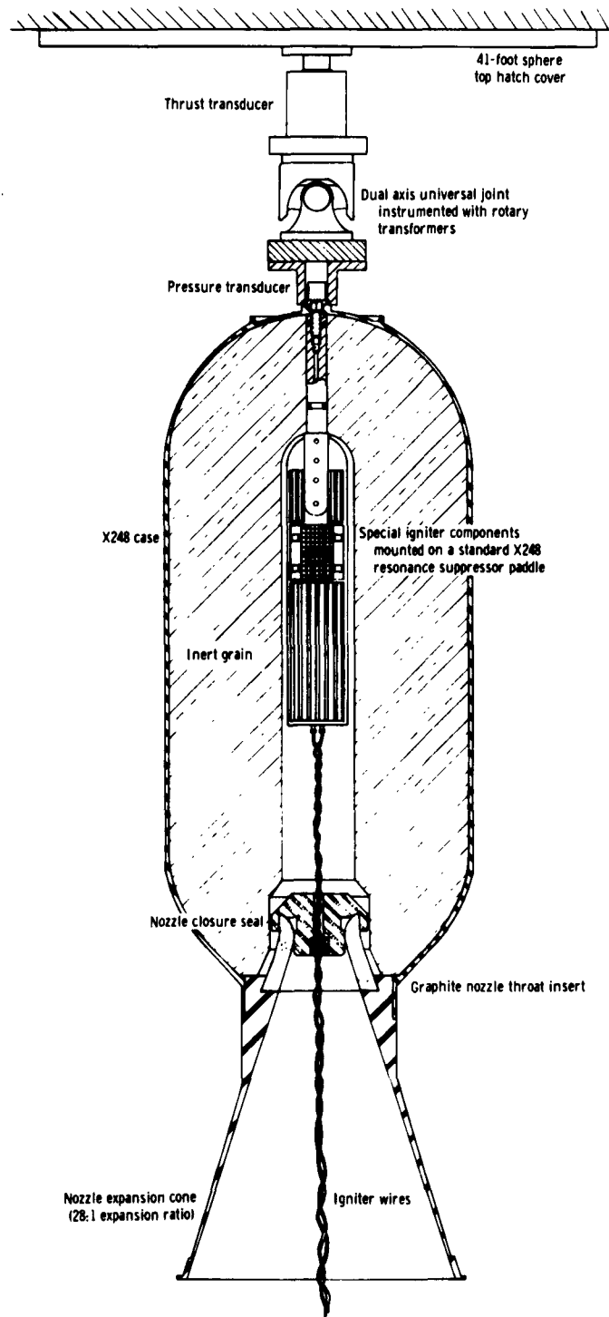
Figure 2.- Schematic illustration of basic test assembly.
