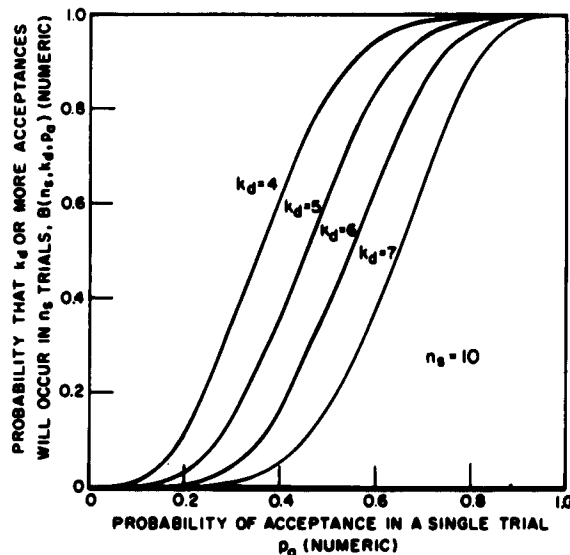
Fig. 8 - Acceptance criterion [B(n_s, k_d, p_a)] vs the probability of acceptance for four values of k_d
