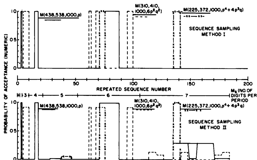
Fig. 18 - Effect of repeated sequences on three measure functions
