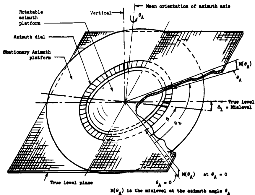
FIG. 4. Mislevel and the Mean Orientation of the Azimuth Axis.
