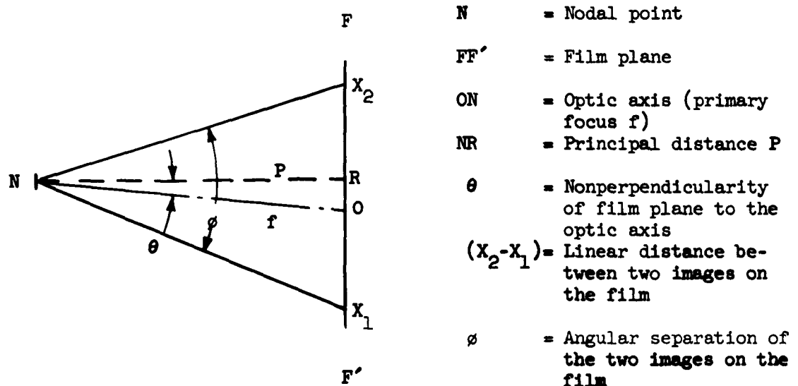
FIG. 2. Principal Distance.
