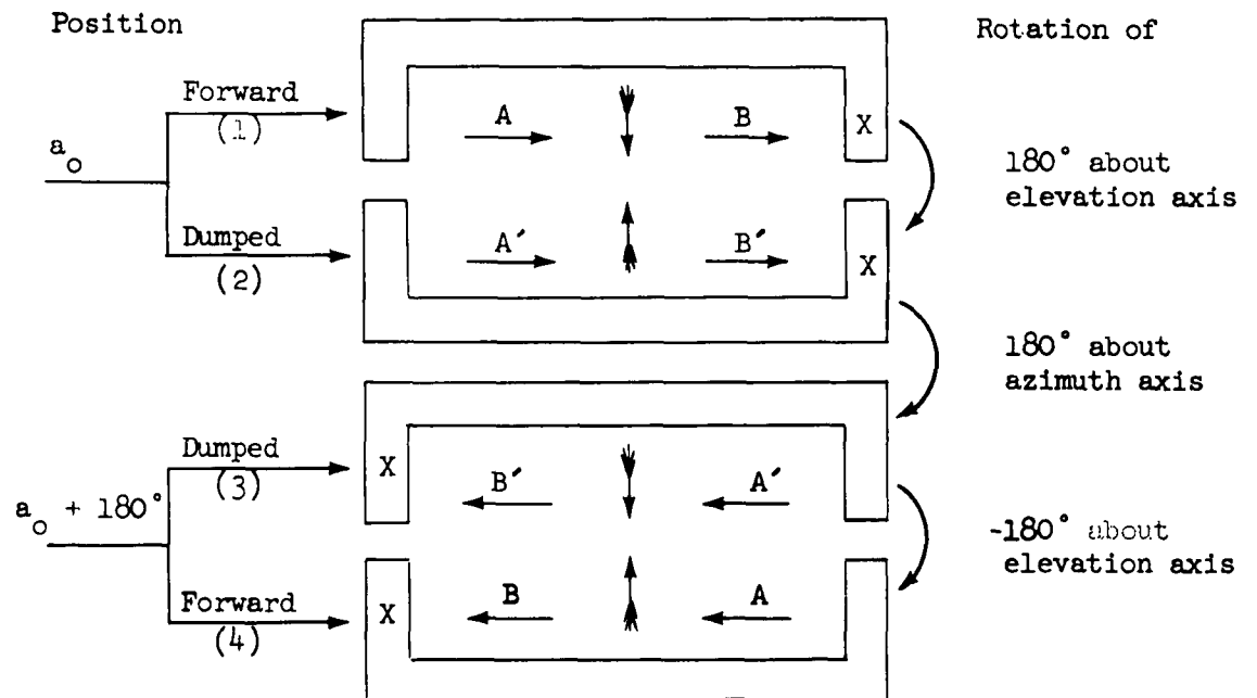
FIG. 12b. Using the Reversion Level Vial.
