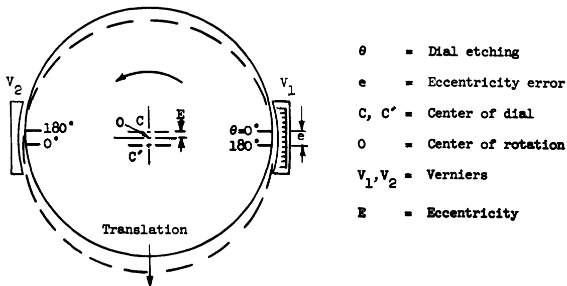
FIG. 3. Dial Eccentricity.
