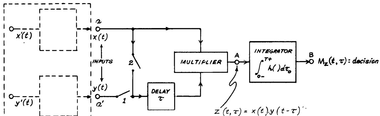
Figure 1. Simple Correlation detectors
