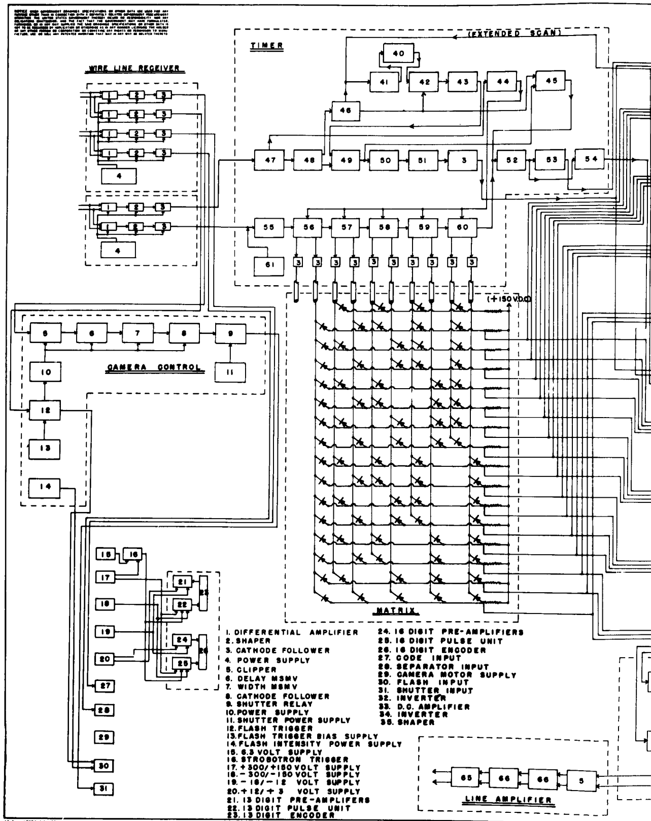
Figure 20. Block Diagram of Field
