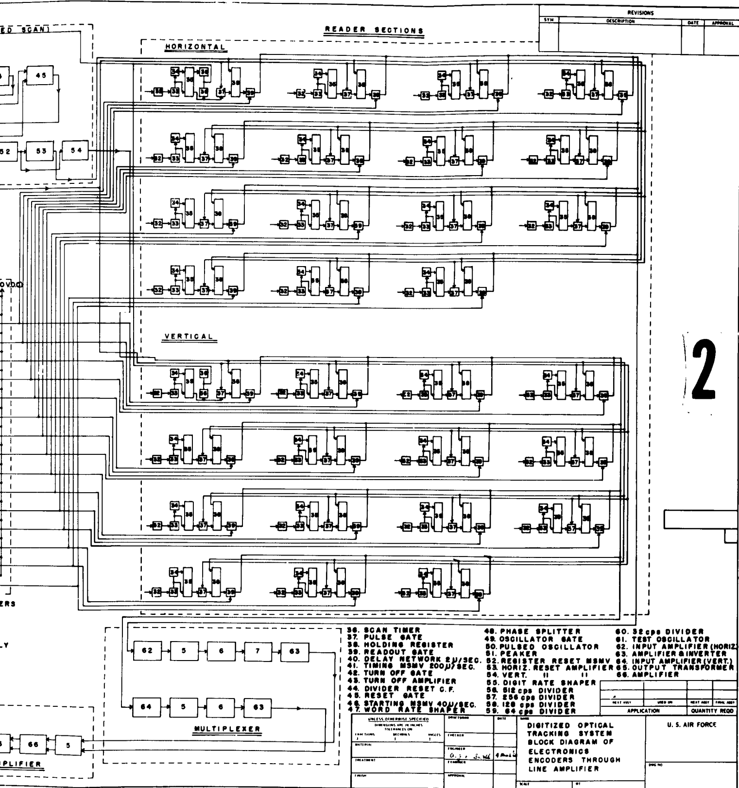
Block Diagram of Field Station Electronics
