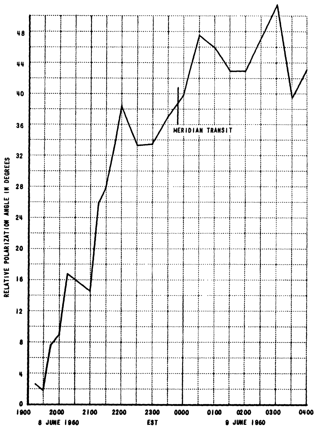
Figure 15 DIURNAL VARIATION OF THE LUNAR ECHO POLARIZATION 8 - 9 JUNE 1960
