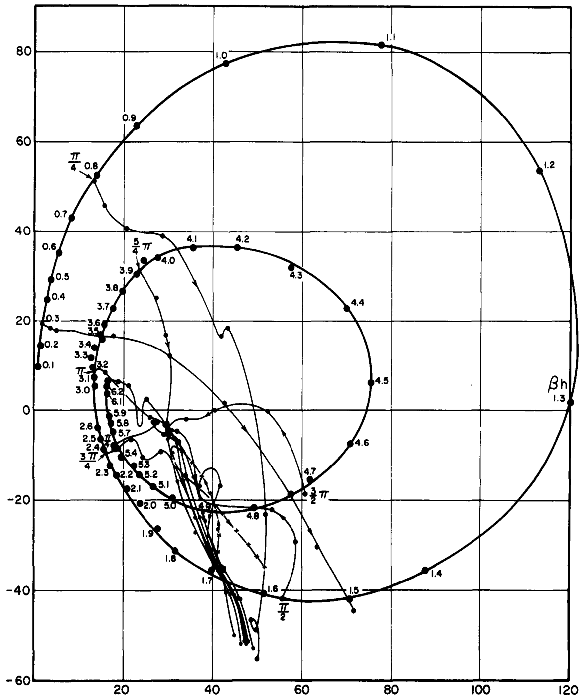
FIG. 3-11 LOCI OF ADMITTANCE WITH THE CHANGE OF CONDUCTIVITY
