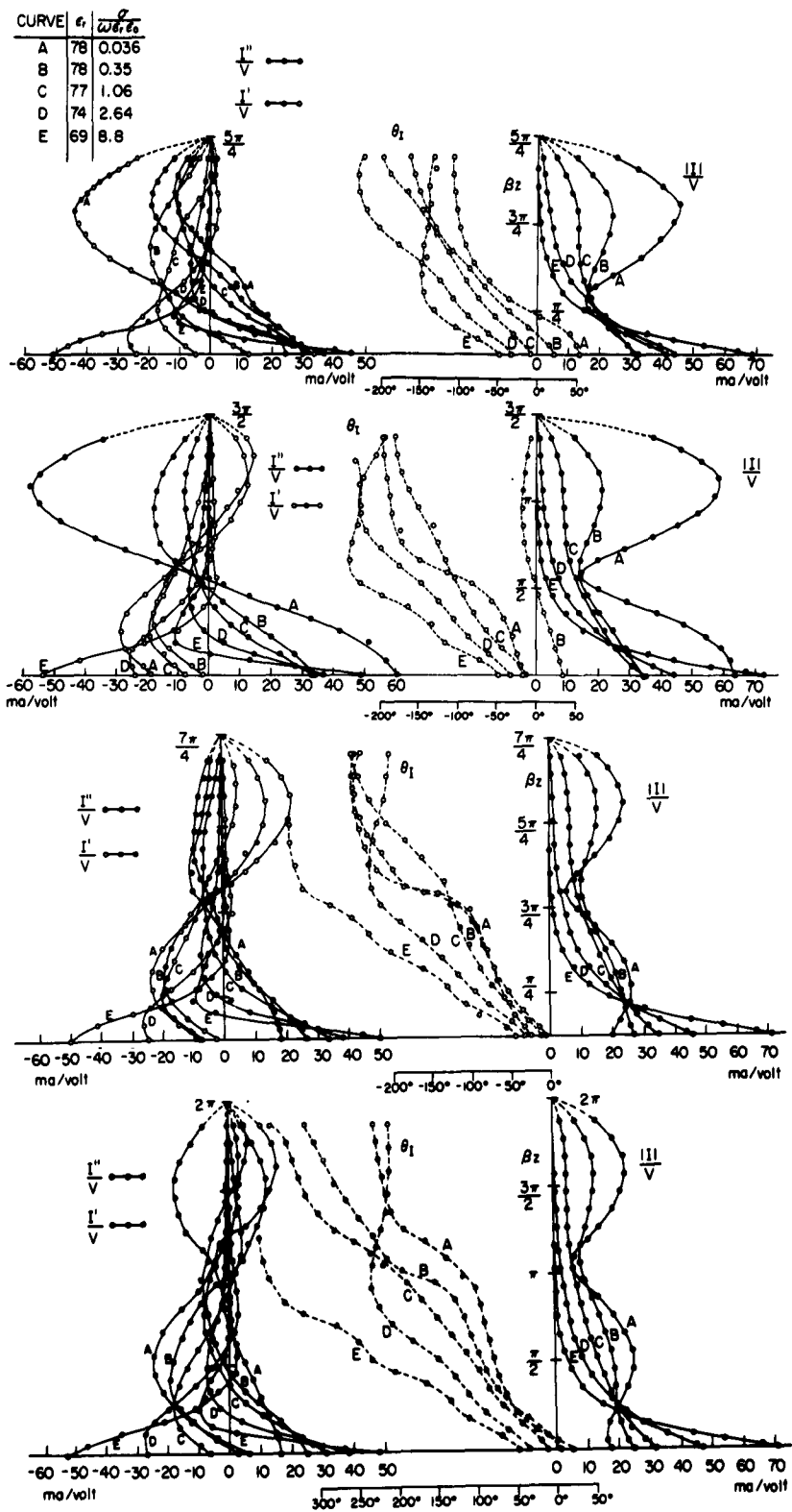
FIG. 3-19(b) CURRENT DISTRIBUTION \frac{I}{V} = \frac{II}{V} e^{i\theta_1} = \frac{I''}{V} + j \frac{I'}{V} ALONG ANTENNAS \beta_h = \frac{5\pi}{4}, \frac{3\pi}{2}, \frac{7\pi}{4}, 2\pi IN SOLUTIONS WITH VARIOUS CONDUCTIVITIES.
