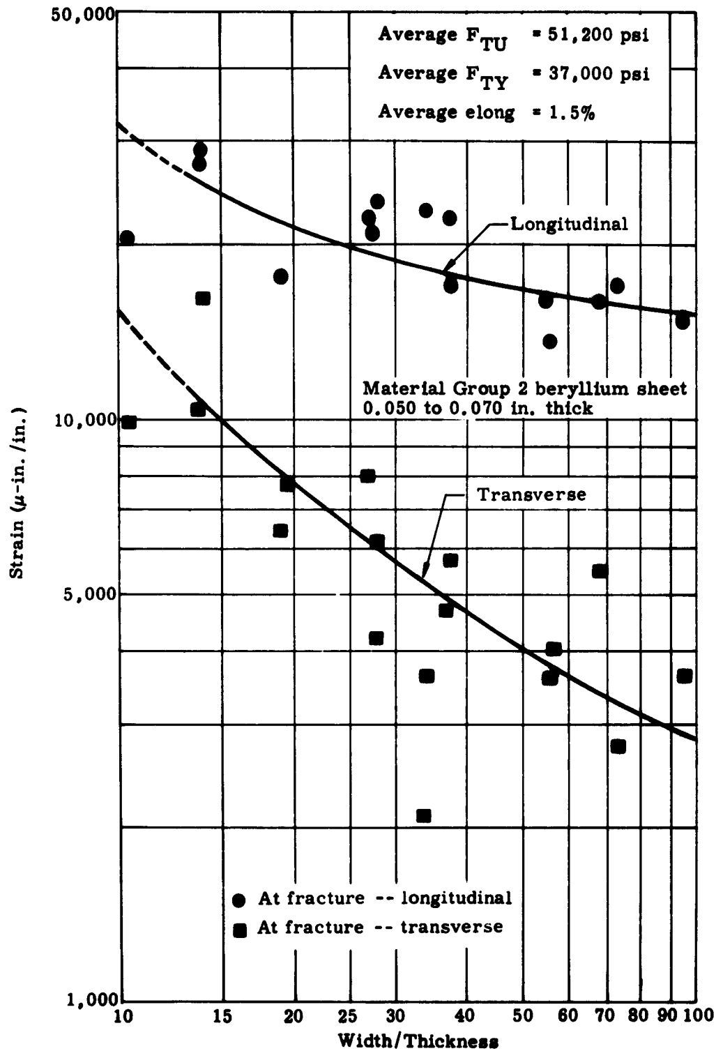
Fig. 11. Variation of Maximum Strain with Size in a Constant Moment Bend Test, Group 2, Beryllium Sheet (Hot-Pressed)
