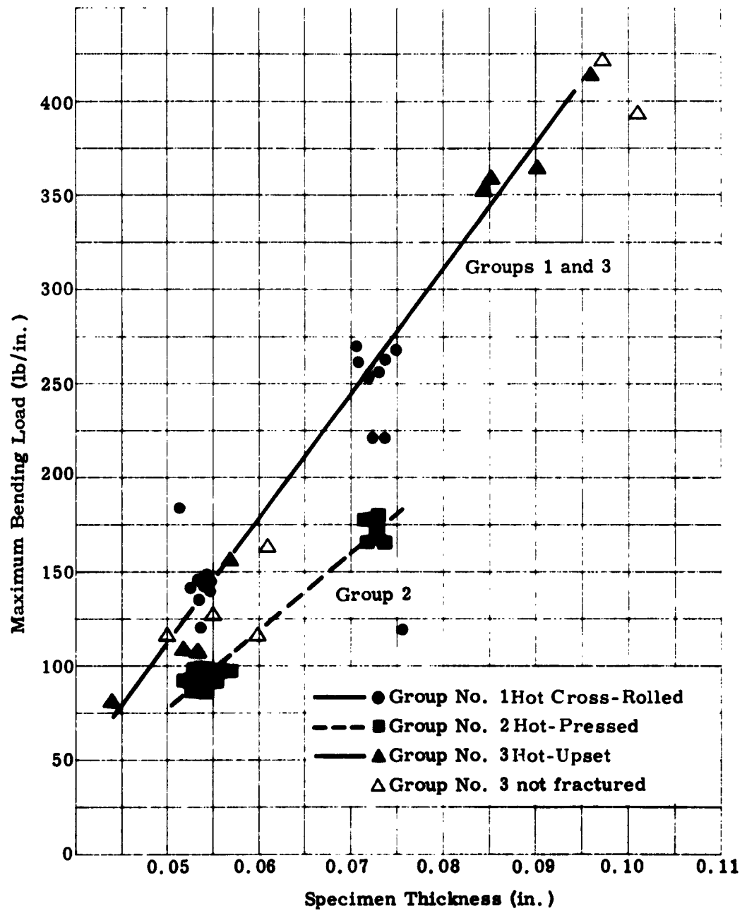
Fig. 9. Variation of Maximum Bending Load with Thickness for the Beryllium Bend Ductility Specimens
