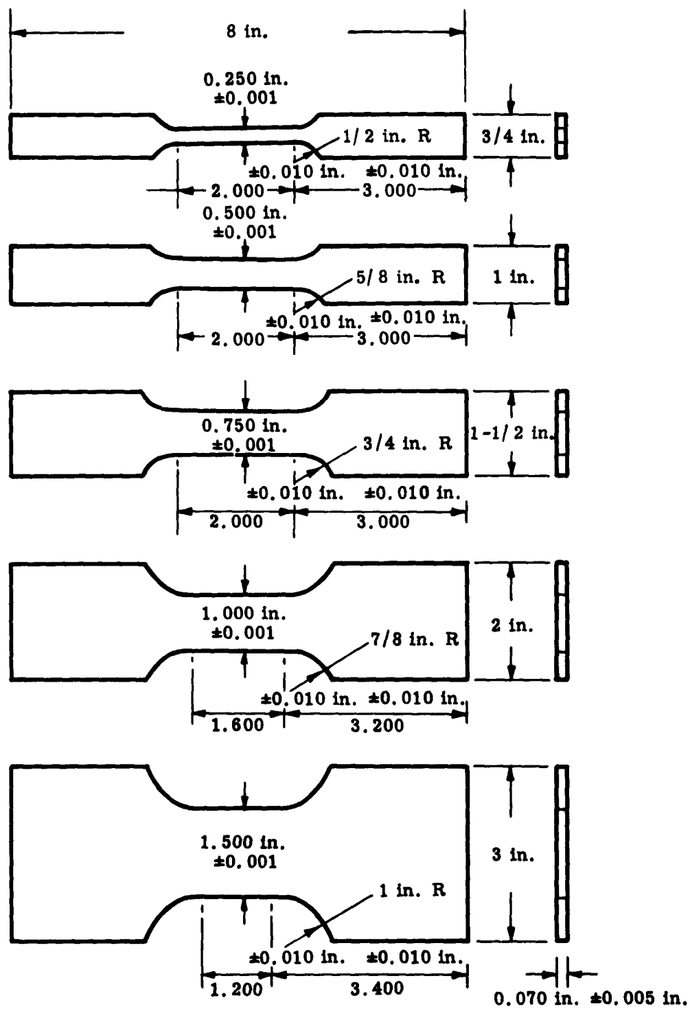
Fig. 1. Tension Specimens, Specifications
