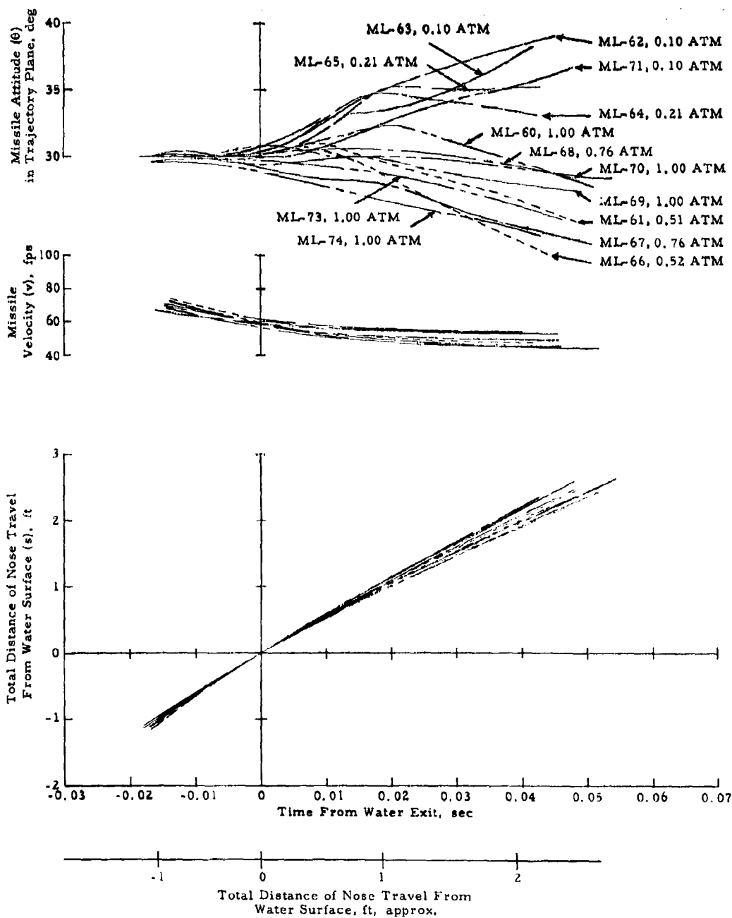
FIG. 15. Effect of Atmospheric Pressure on Water-Exit Behavior of Missile Without Probe Launched at 30-deg Angle.
