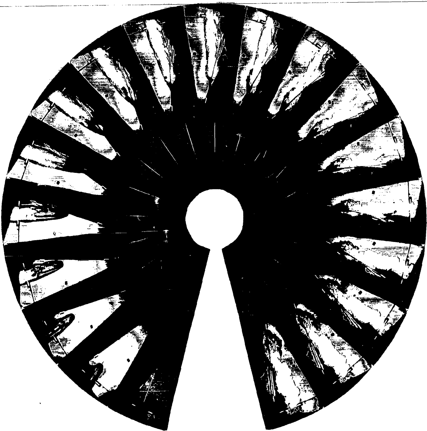
FIG. 18. Erratic Cavity Caused by Addition of Probe to Missile. (ML 97, velocity 63.3 fps, pressure 0.1 atm.)
