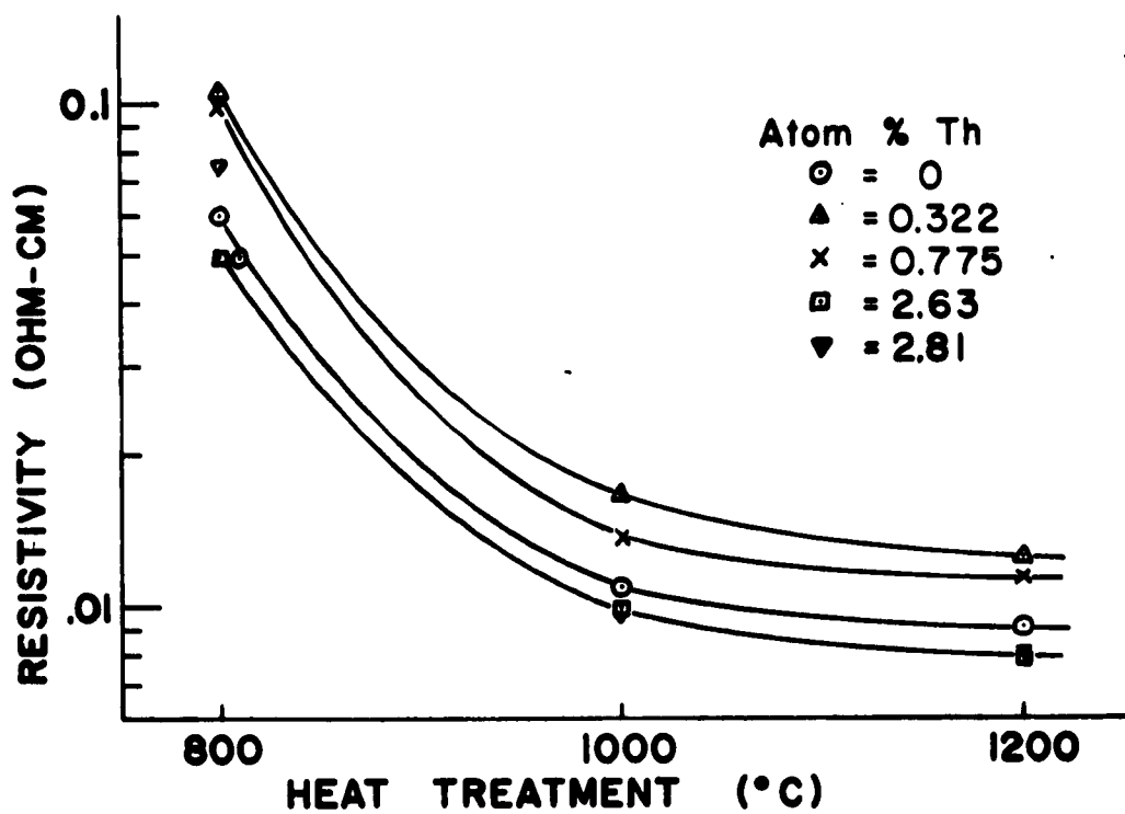
Fig. 3 Variation of pellet resistivity (uncorrected) with pyrolysis temperature.
